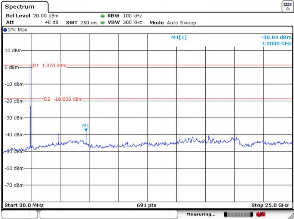
GFSK 2402 MHz
