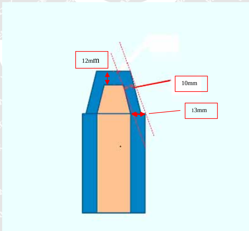
A(antenna location and the distances from antenna to head edge)
