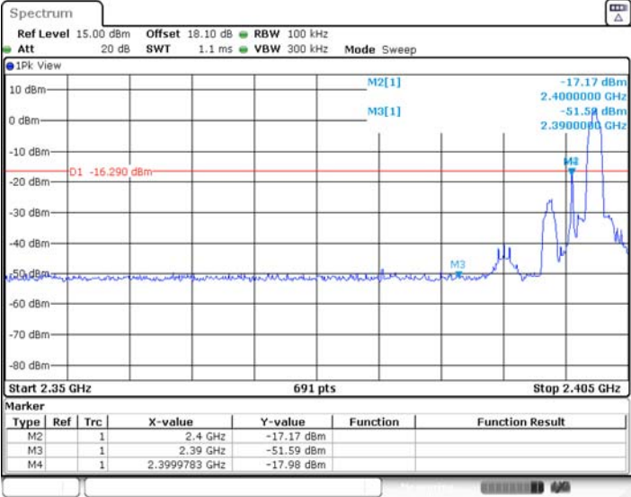
2DH5_Ant1_Low_2402
