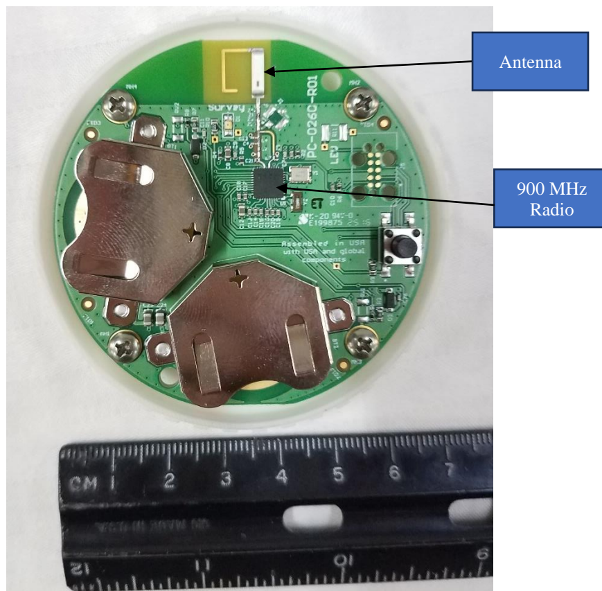
Figure 2. Main PCB, Front
