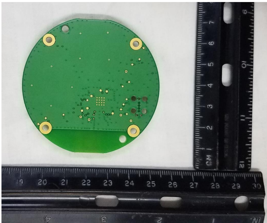
Figure 3. Main PCB Back Side
