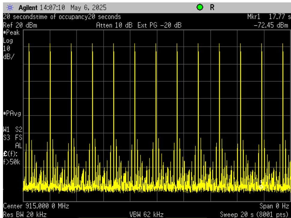
Figure 21. Average Time of Occupancy
