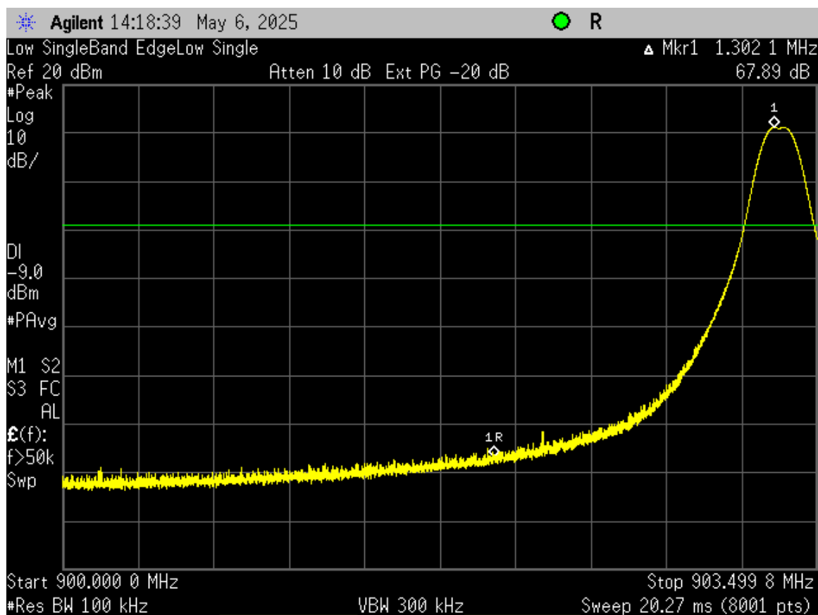
Figure 9. Band Edge Compliance, Low Channel Delta – Hopping Off
