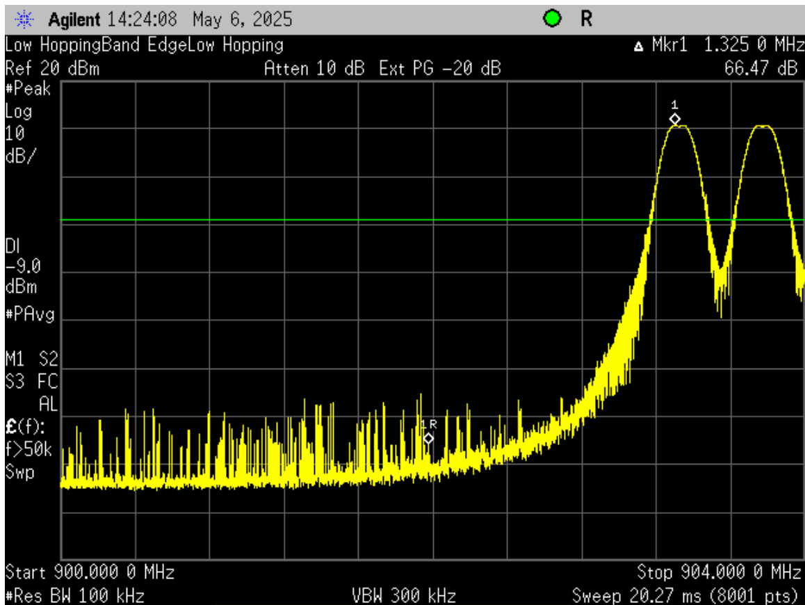
Figure 10. Band Edge Compliance, Low Channel Delta – Hopping On
