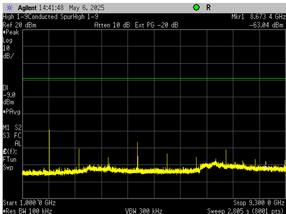
Figure 8. Antenna Conducted Emissions, High Channel 1000 MHz – 9300 MHz
