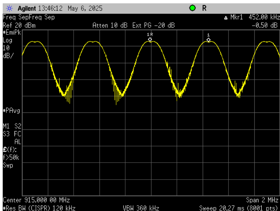
Figure 20. Channel Separation
