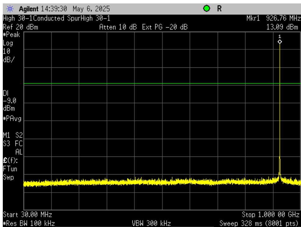
Figure 7. Antenna Conducted Emissions, High Channel 30 MHz to 1000 MHz
