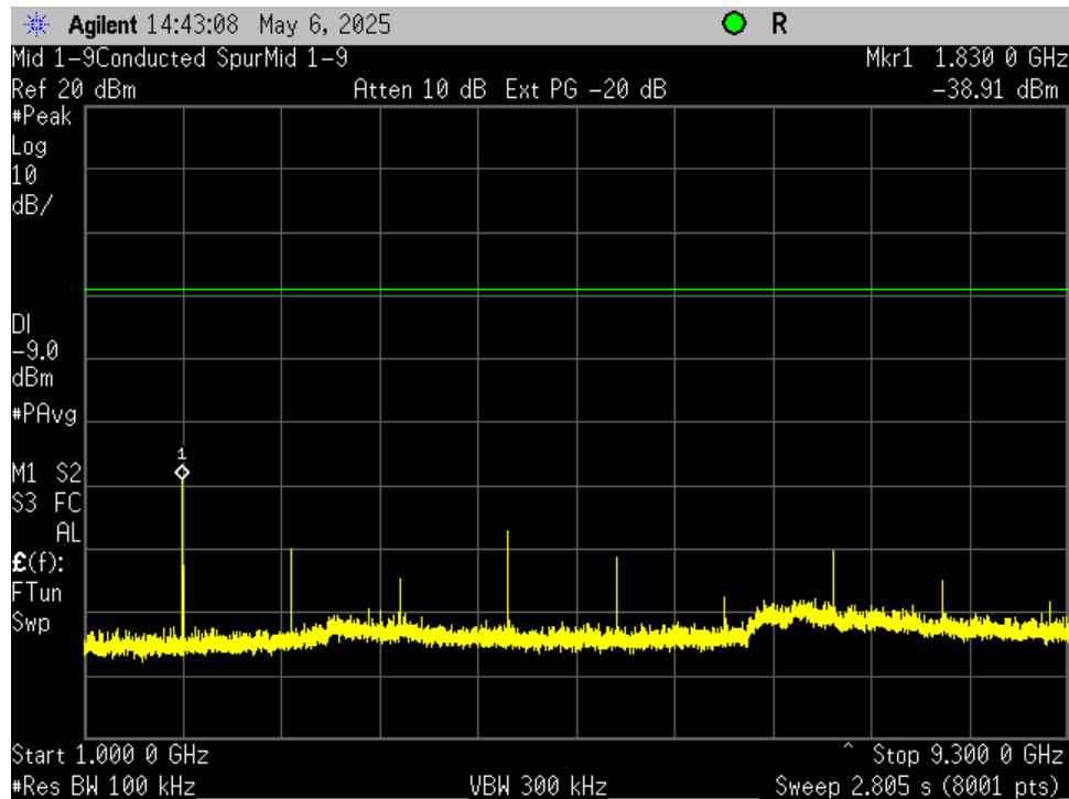
Figure 6. Antenna Conducted Emissions, Middle Channel 1000 MHz – 9300 MHz
