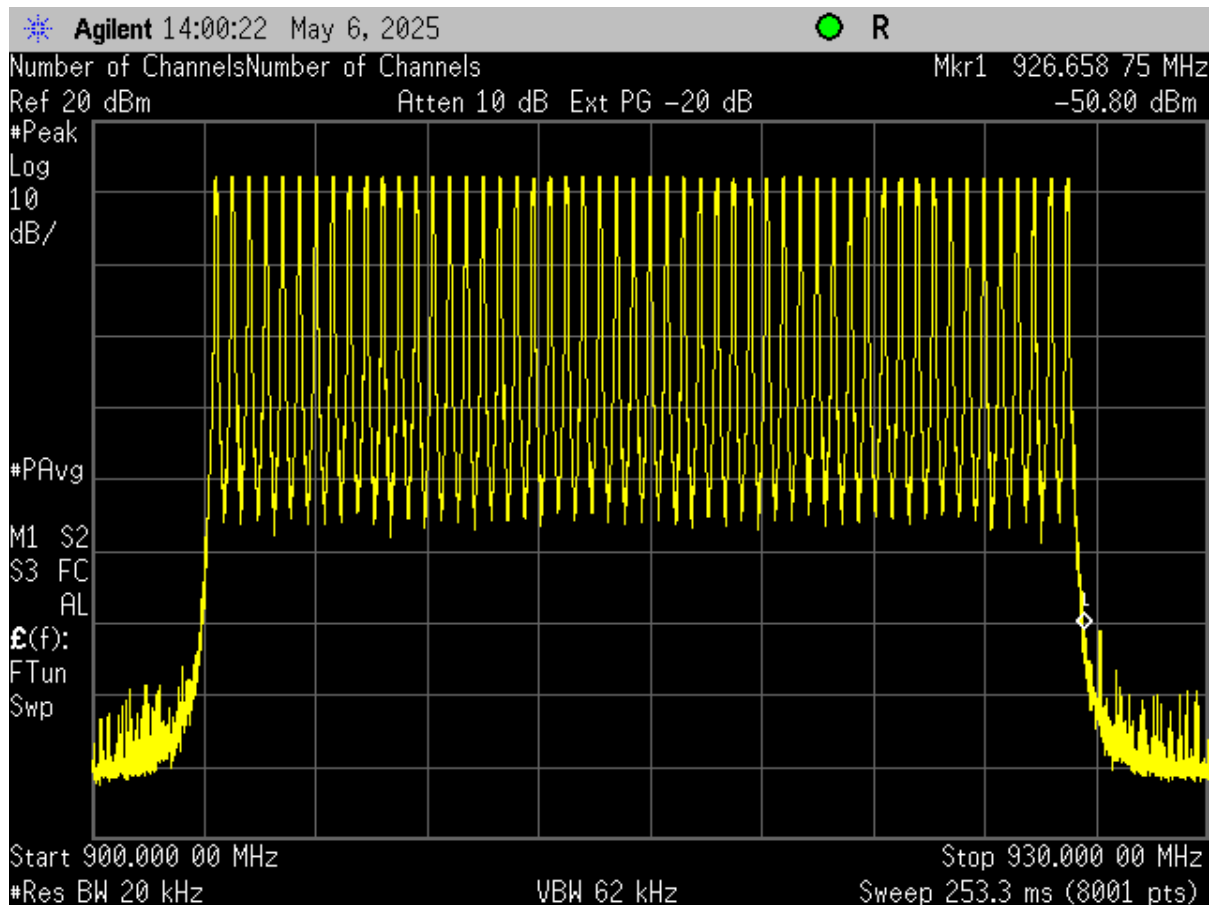
Figure 16. Hopping Channels 0 through 52
