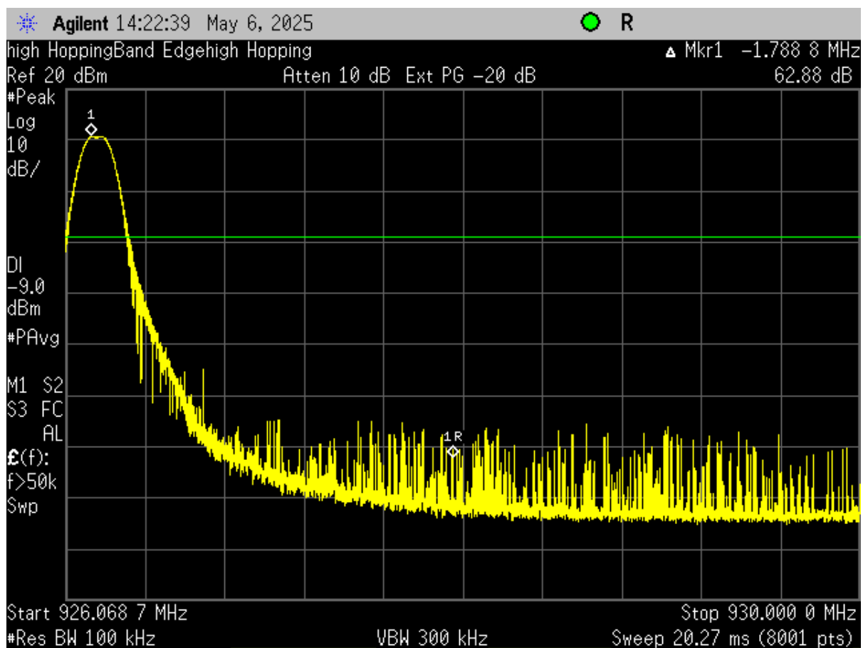
Figure 12. Band Edge Compliance, High Channel Delta – Hopping On
