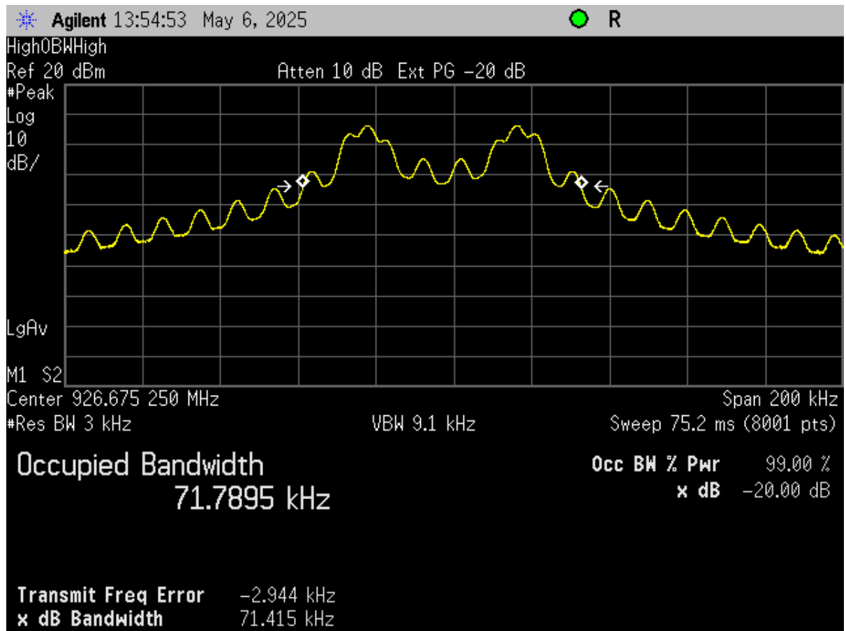
Figure 15. Twenty dB Bandwidth – High Channel
