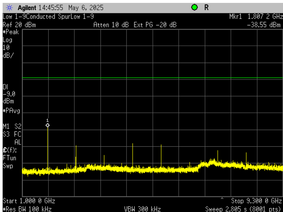
Figure 4. Antenna Conducted Emissions, Low Channel 1000 MHz to 9300 MHz
