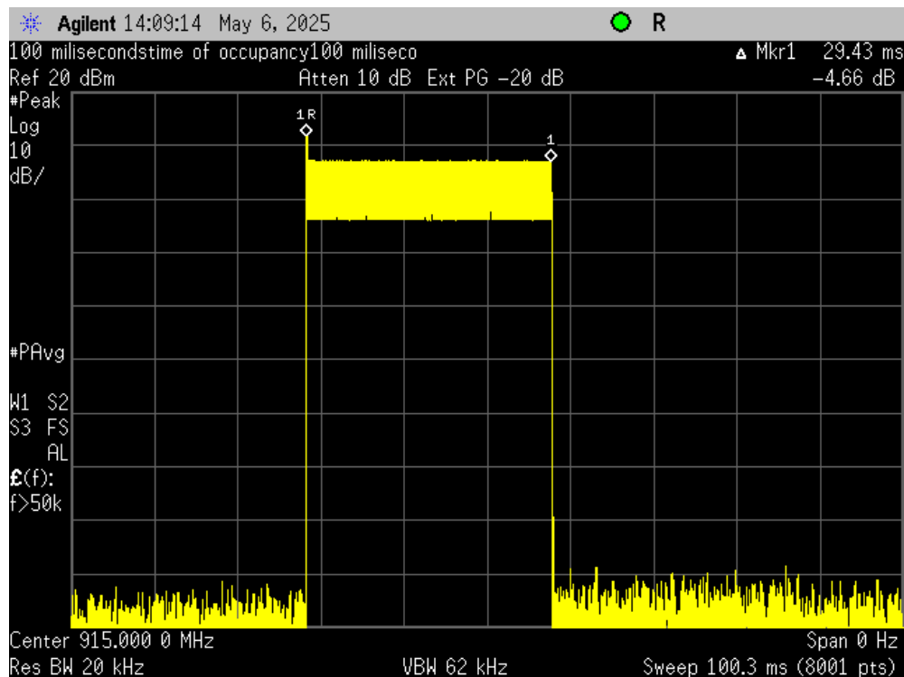
Figure 2. Duty Cycle 100ms Sweep
