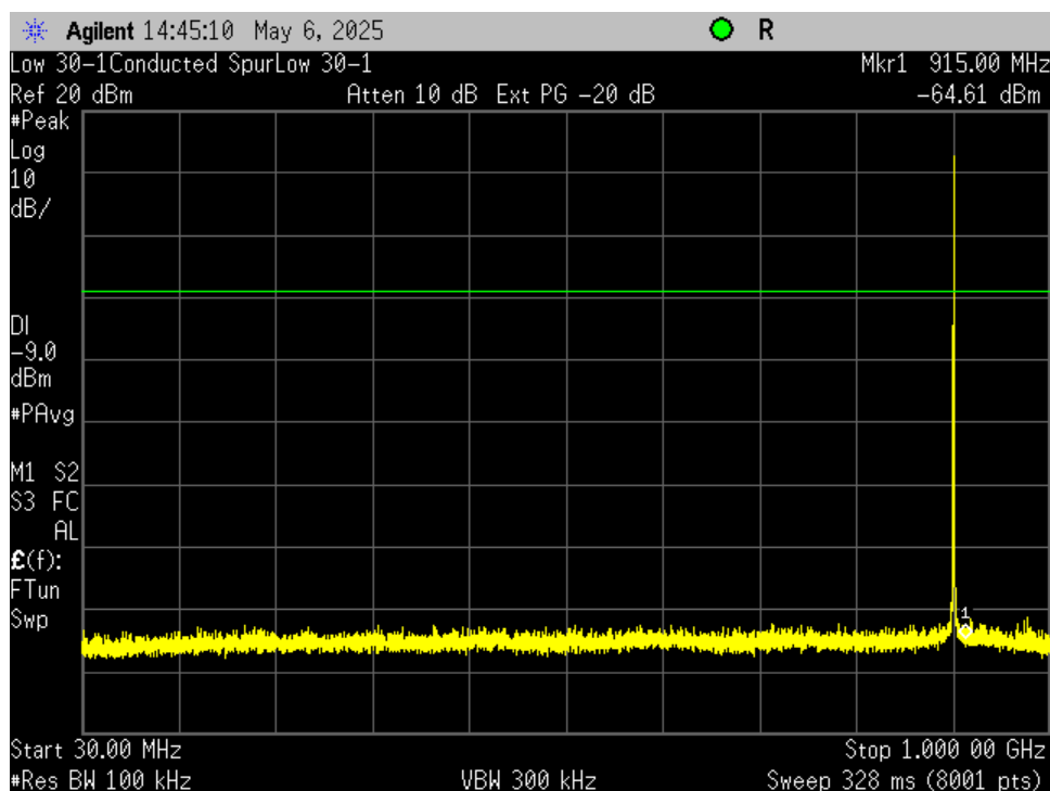
Figure 3. Antenna Conducted Emissions, Low Channel 30 MHz to 1000 MHz
