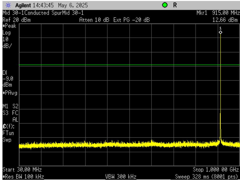
Figure 5. Antenna Conducted Emissions, Middle Channel 30 MHz to 1000 MHz
