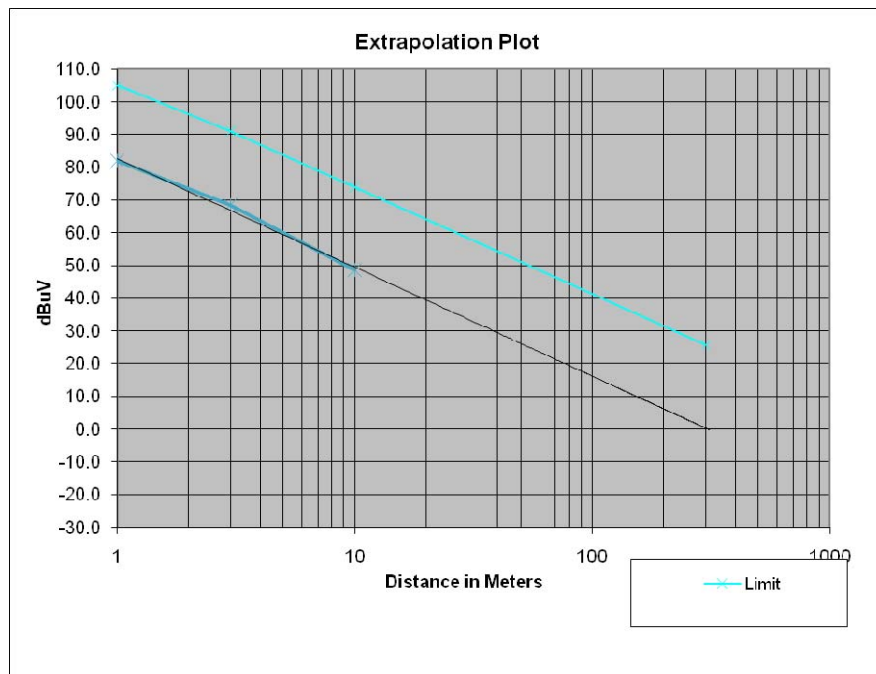
Figure Nine Extrapolated Radiated Emissions data.
