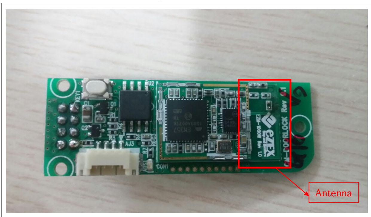
Zigbee Board - Front
