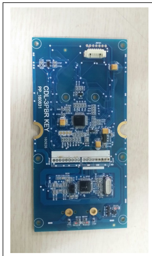
Touch Board - Rear
