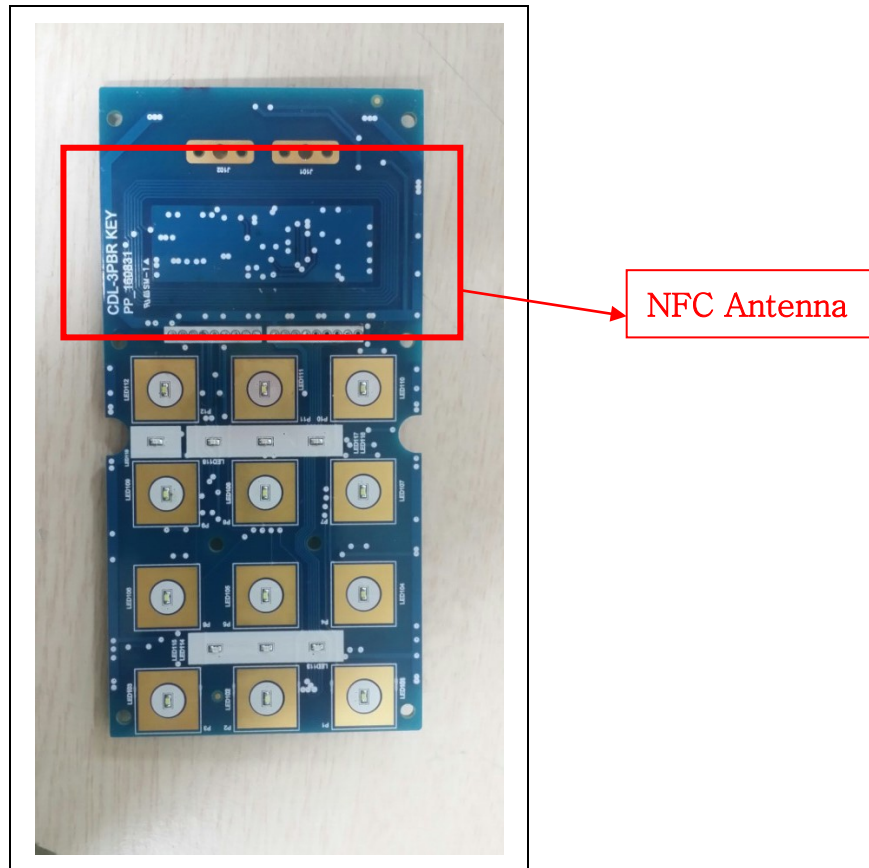
Touch Board - Rear
