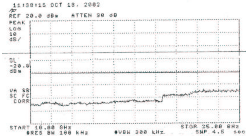
Figure 6.5 Antenna Conducted Spurious Emissions. (all channels)
