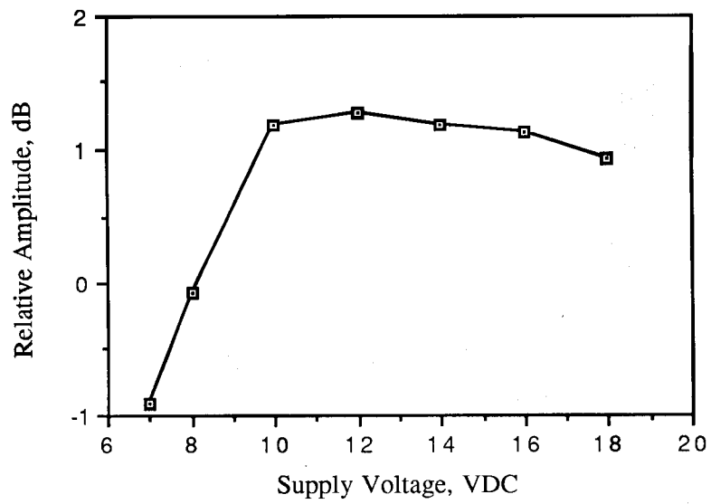
Figure 6.4. Relative emission vs. supply voltage. (310 MHz, CW)
