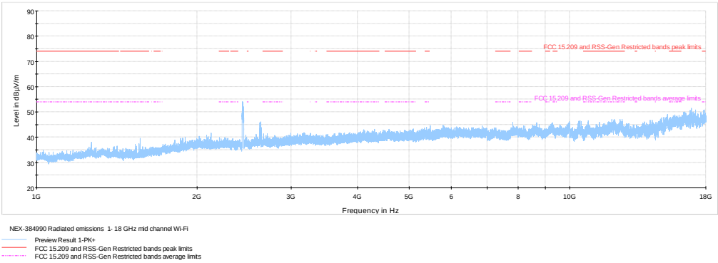
Figure 8.5-17: Radiated spurious emissions within 1–18 GHz, mid channel
