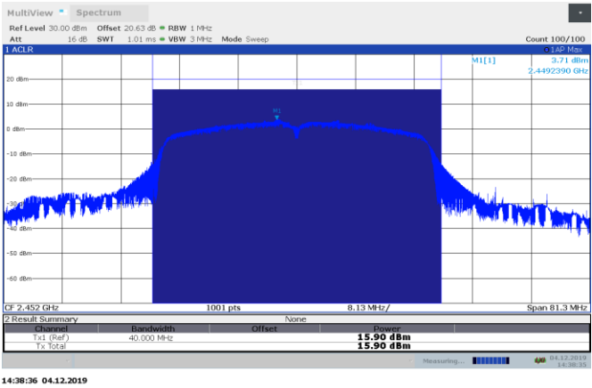
Figure 8.4-4: Conducted output power on 802.11n HT40, sample plot
