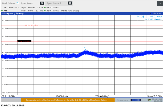
Figure 8.5-20: Radiated spurious emissions above 18 GHz, mid channel
