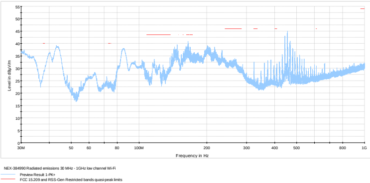
Figure 8.5-13: Radiated spurious emissions below 1 GHz, low channel
