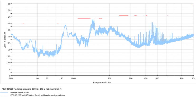
Figure 8.5-14: Radiated spurious emissions below 1 GHz, mid channel
