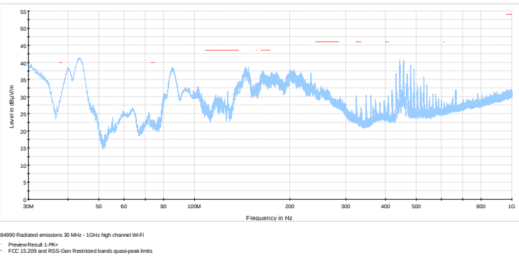
Figure 8.5-15: Radiated spurious emissions below 1 GHz, high channel
