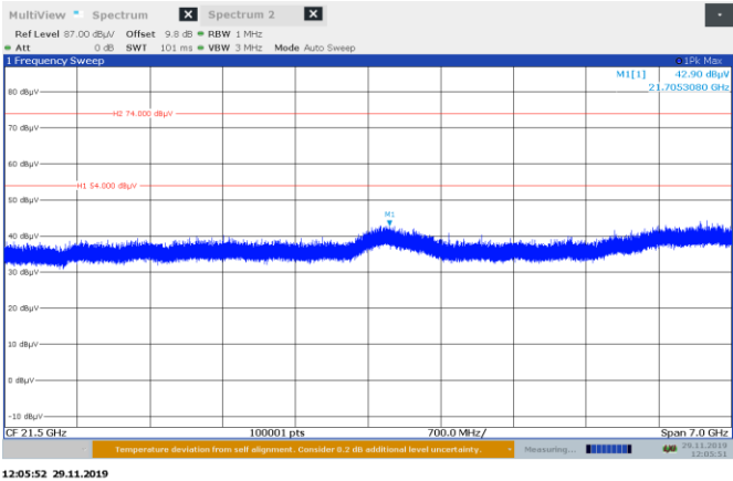
Figure 8.5-19: Radiated spurious emissions above 18 GHz, low channel
