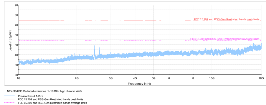
Figure 8.5-18: Radiated spurious emissions within 1-18 GHz, high channel
