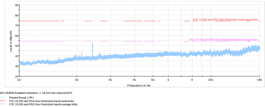
Figure 8.5-16: Radiated spurious emissions within 1–18 GHz, low channel
