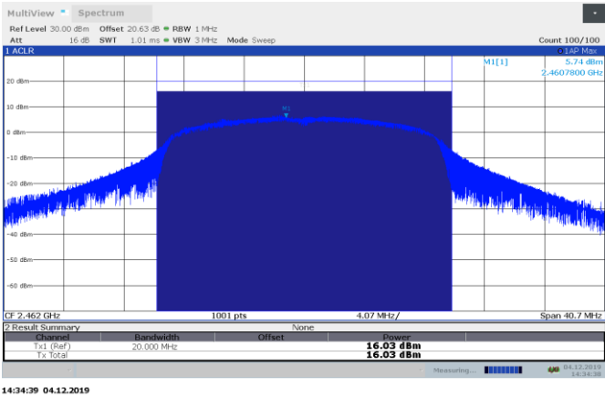
Figure 8.4-3: Conducted output power on 802.11n HT20, sample plot
