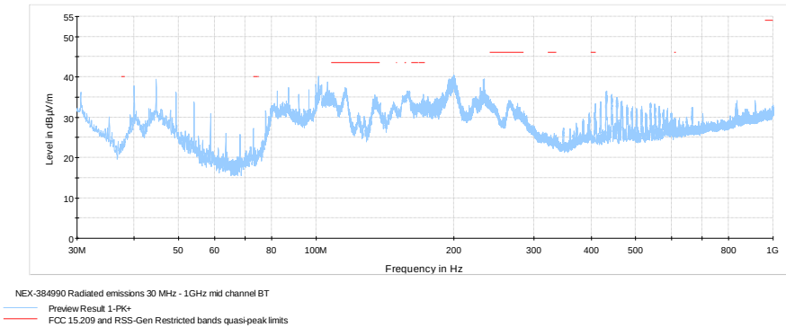
Figure 8.6-28: Radiated spurious emissions below 1 GHz, mid channel
