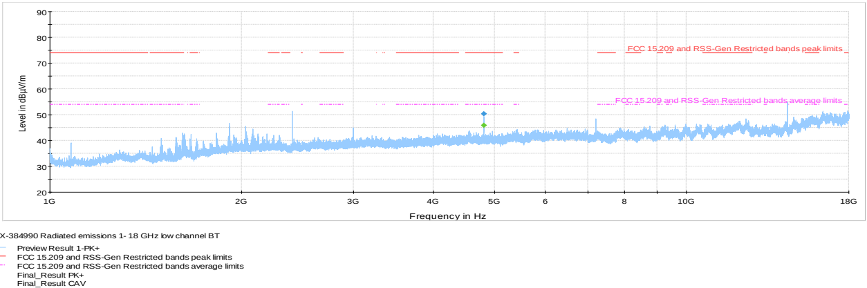
Figure 8.6-30: Radiated spurious emissions within 1–18 GHz, low channel
