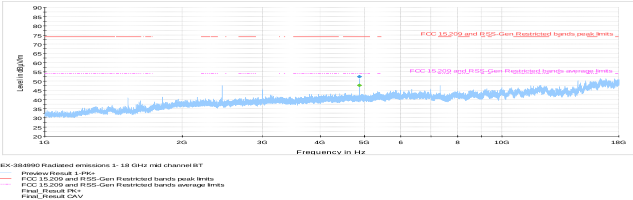
Figure 8.6-31: Radiated spurious emissions within 1–18 GHz, mid channel
