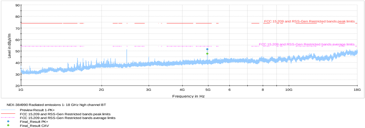
Figure 8.6-32: Radiated spurious emissions within 1-18 GHz, high channel
