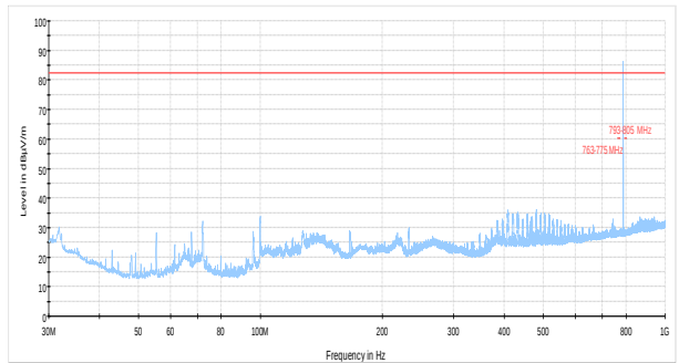
Figure 8.3-7: Radiated spurious below 1GHz high channel 787.9875 MHz analogue voice
