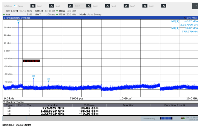
Figure 8.2-17: Conducted spurious emissions 9 kHz – 10 GHz low channel 776.0125 MHz DMR
