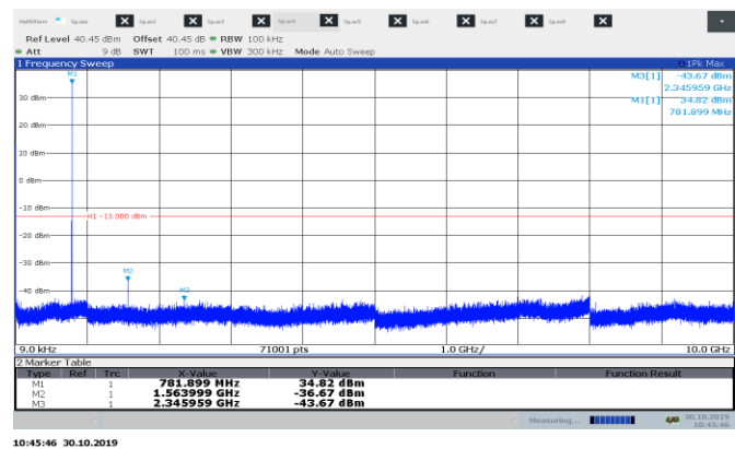
Figure 8.2-18: Conducted spurious emissions 9 kHz – 10 GHz mid channel 782 MHz DMR
