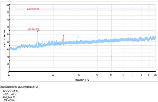
Figure 8.3-16: Radiated spurious above 1GHz mid channel 782 FFSK
