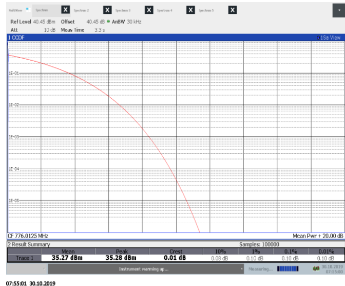
Figure 8.1-2: CCDF sample plot for PAPR values
