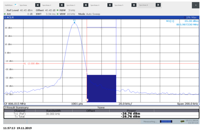
Figure 8.2-29: High band edge for emissions outside operating band in high channel 805.9875 MHz analogue FM
