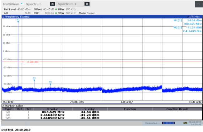
Figure 8.2-34: Conducted spurious emissions 9 kHz – 10 GHz mid channel 805.5 MHz analogue FM
