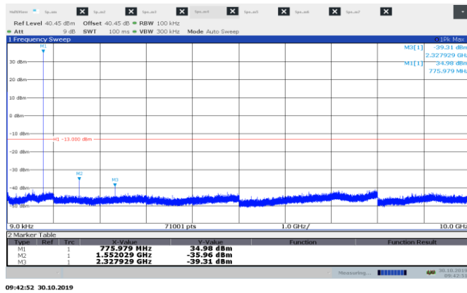
Figure 8.2-15 : Conducted spurious emissions 9 kHz – 10 GHz low channel 776.0125 MHz FFSK
