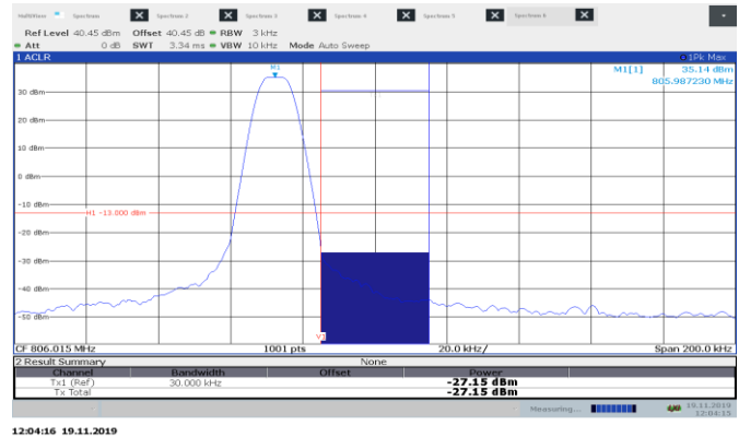
Figure 8.2-33: : High band edge for emissions outside operating band in high channel 805.9875 MHz DMR
