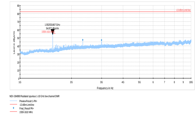
Figure 8.3-17 Radiated spurious above 1GHz low channel 776.0125 MHz DMR
