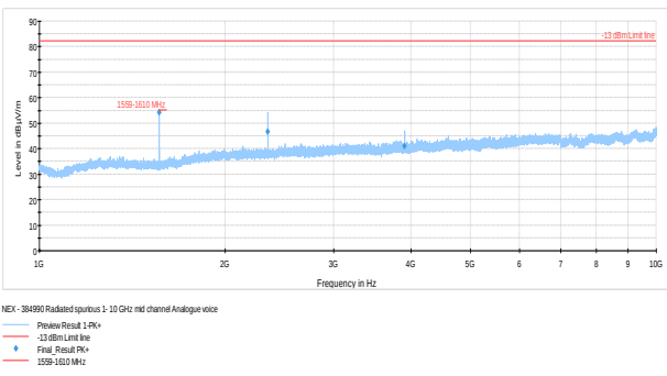
Figure 8.3-14: Radiated spurious above 1GHz mid channel 782 MHz analogue voice
