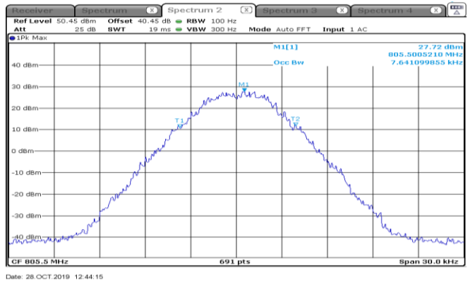
Figure 8.8-6: OBW plot for 805.5 MHz DMR
