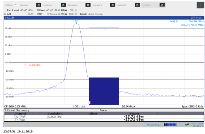
Figure 8.2-31: High band edge for emissions outside operating band in high channel 805.9875 MHz FFSK
