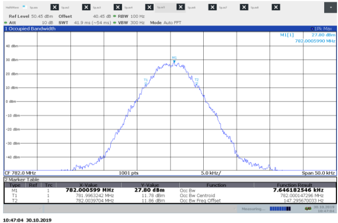
Figure 8.8-5: OBW plot for 782 MHz DMR
