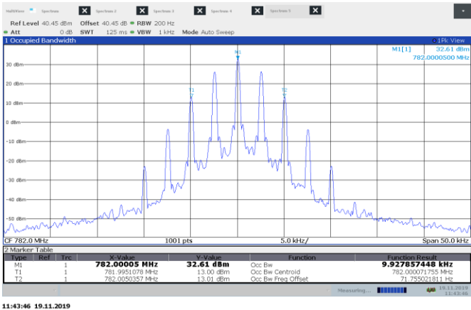
Figure 8.8-1:OBW plot for 782 MHz Analogue FM
