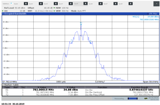
Figure 8.8-3: OBW plot for 782 MHz FFSK
