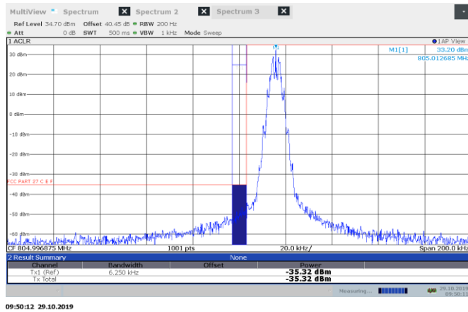
Figure 8.2-30 : Band edge on 805 MHz for protection band 788-805 MHz low channel 805.0125 MHz FFSK
