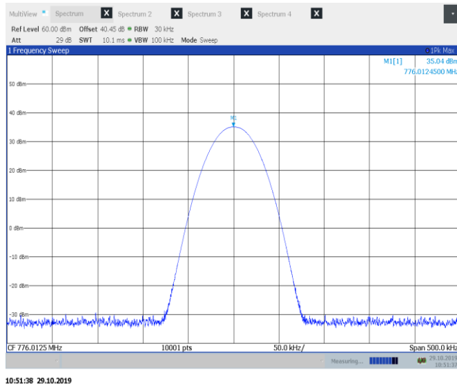
Figure 8.1-1: Output power sample plot
