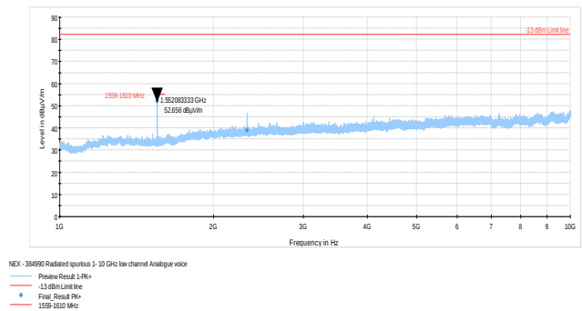
Figure 8.3-13: Radiated spurious above 1GHz low channel 776.0125 MHz analogue voice
