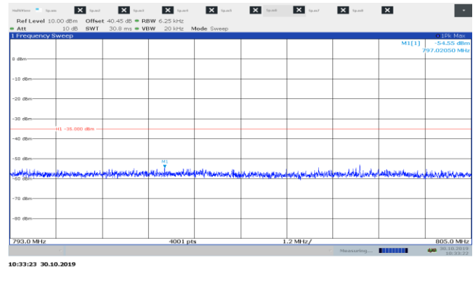
Figure 8.2-4: Spurious emissions within 793-805 MHz protection band for high channel 787.9875 MHz FFSK
