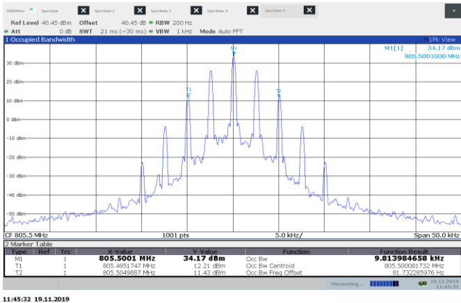
Figure 8.8-2: OBW plot for 805.5 MHz Analogue FM
