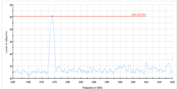
Figure 8.4-1: Field strength within 1559-1610 MHz band 786.9875 MHz analogue voice
