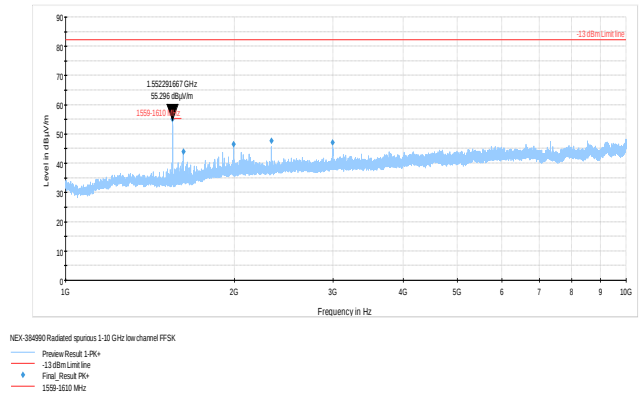
Figure 8.3-15 Radiated spurious above 1GHz low channel 776.0125 MHz FFSK
