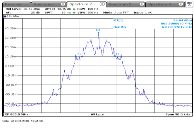
Figure 8.8-4: OBW plot for 805.5 MHz FFSK
