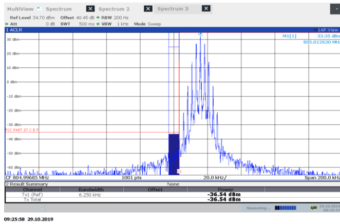
Figure 8.2-28: Band edge on 805 MHz for protection band 788-805 MHz low channel 805.0125 MHz analogue FM
