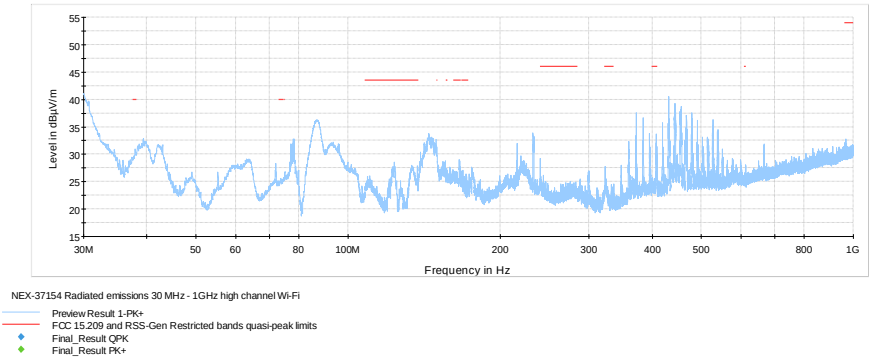
Figure 8.5-15: Radiated spurious emissions below 1 GHz, high channel
