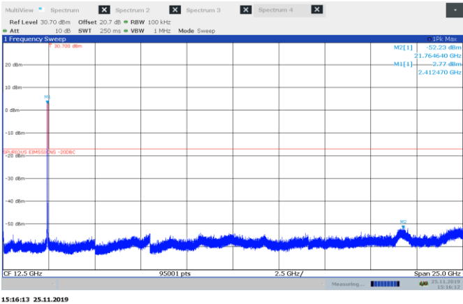
Figure 8.5-1: Conducted spurious emissions for 802.11 b, low channel
