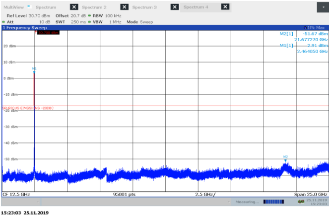
Figure 8.5-3: Conducted spurious emissions for 802.11 b, high channel
