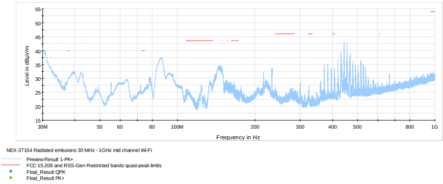
Figure 8.5-14: Radiated spurious emissions below 1 GHz, mid channel
