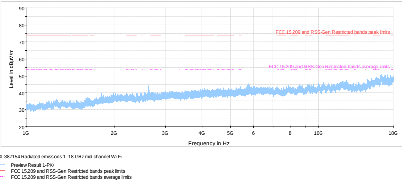
Figure 8.5-17: Radiated spurious emissions within 1–18 GHz, mid channel
