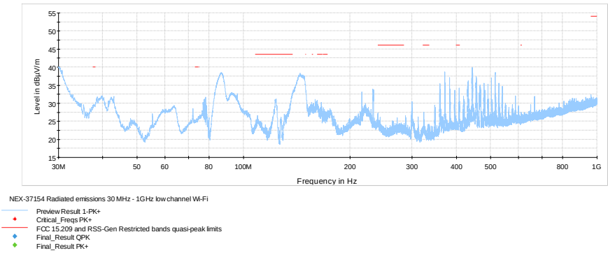
Figure 8.5-13: Radiated spurious emissions below 1 GHz, low channel
