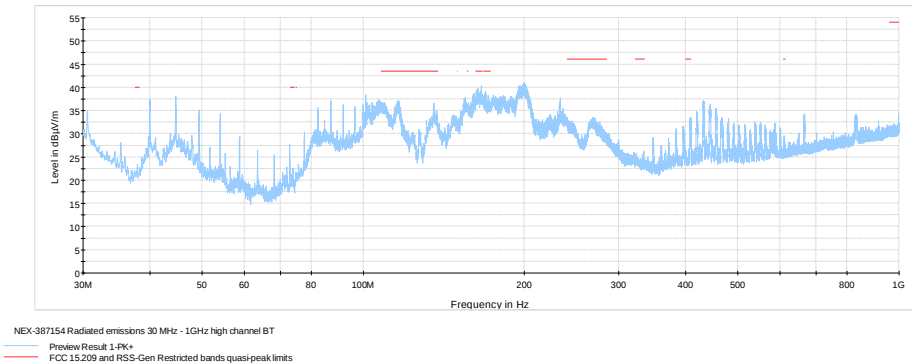
Figure 8.6-29: Radiated spurious emissions below 1 GHz, high channel
