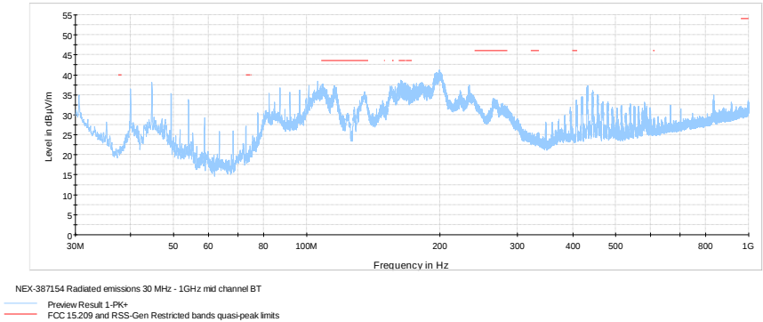
Figure 8.6-28: Radiated spurious emissions below 1 GHz, mid channel
