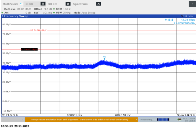
Figure 8.6-34: Radiated spurious emissions above 18 GHz, mid channel
