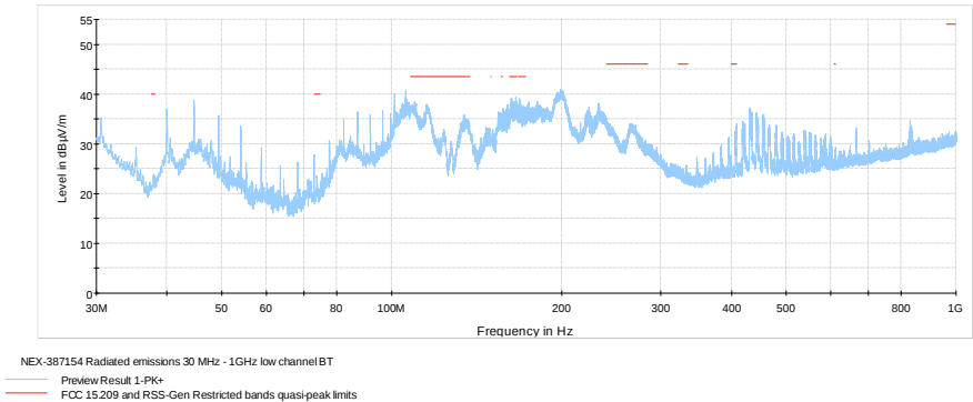
Figure 8.6-27: Radiated spurious emissions below 1 GHz, low channel
