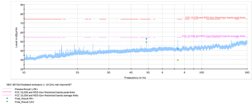
Figure 8.6-31: Radiated spurious emissions within 1-18 GHz, mid channel
