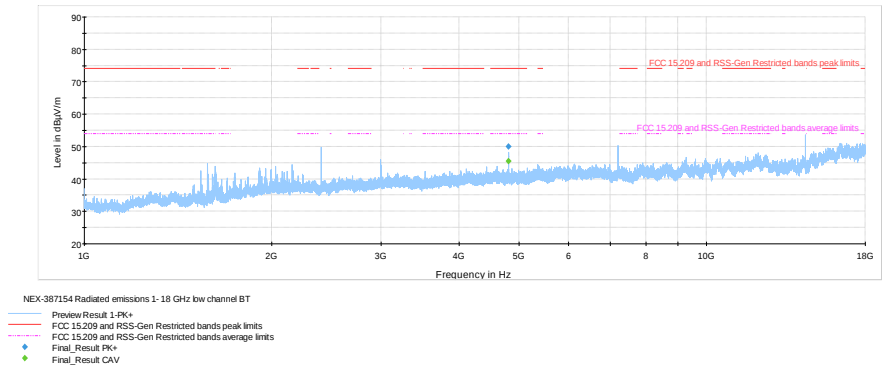
Figure 8.6-30: Radiated spurious emissions within 1-18 GHz, low channel
