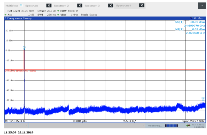
Figure 8.5-6: Conducted spurious emissions for 802.11 g, high channel
