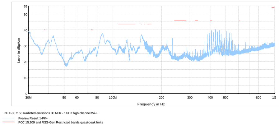
Figure 8.5-15: Radiated spurious emissions below 1 GHz, high channel
