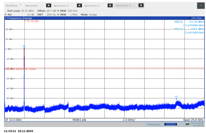
Figure 8.5-8: Conducted spurious emissions for 802.11n 20, mid channel
