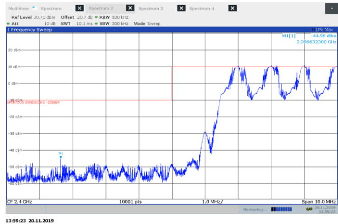
Figure 8.6-2: Conducted spurious emissions at the lower band edge for GFSK modulation, hopping on
