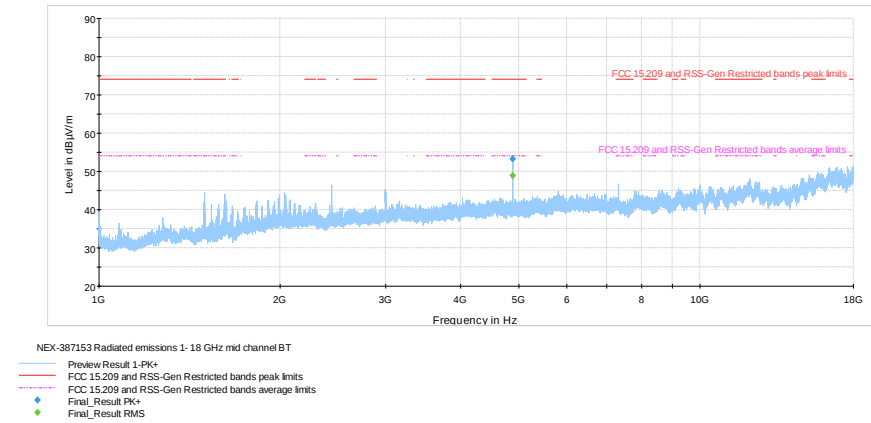
Figure 8.6-31: Radiated spurious emissions within 1-18 GHz, mid channel
