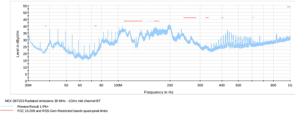
Figure 8.6-28: Radiated spurious emissions below 1 GHz, mid channel
