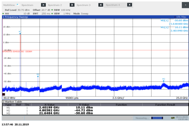
Figure 8.6-15: Conducted spurious emissions for GFSK, low channel
