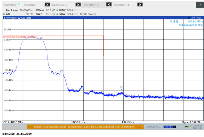
Figure 8.6-13: Conducted spurious emissions at the upper band edge for 8DPSK modulation, hopping off
