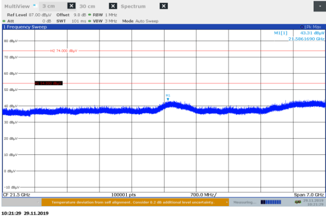
Figure 8.6-34: Radiated spurious emissions above 18 GHz, mid channel
