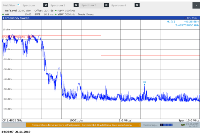
Figure 8.6-12: Conducted spurious emissions at the upper band edge for \pi/4 -DQPSK modulation, hopping on
