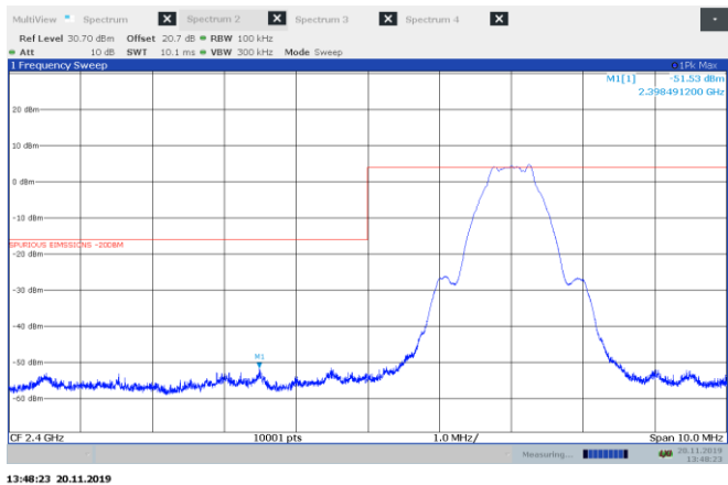
Figure 8.6-7: Conducted spurious emissions at the lower band edge for BLE modulation
