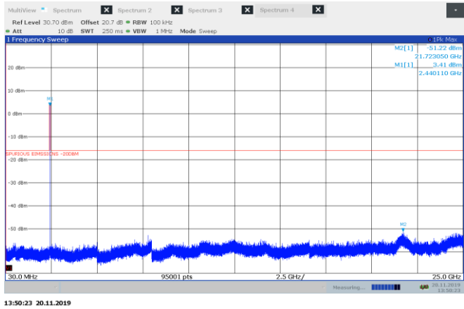
Figure 8.6-25: Conducted spurious emissions for BLE, mid channel
