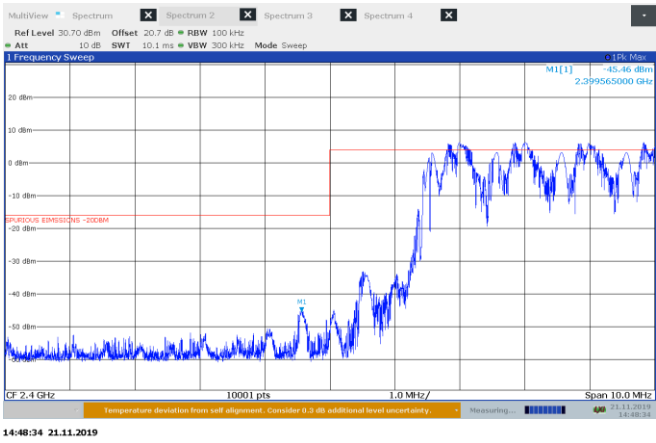
Figure 8.6-6: Conducted spurious emissions at the lower band edge for 8DPSK modulation, hopping on
