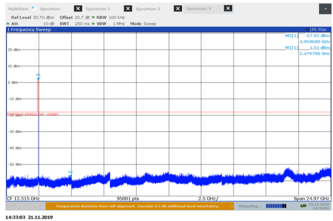
Figure 8.6-20: Conducted spurious emissions for \pi/4 -DQPSK, high channel
