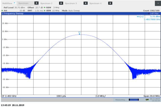
Figure 8.5-1: Output power sample plot
