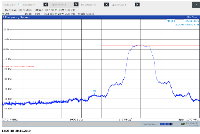
Figure 8.6-5: Conducted spurious emissions at the lower band edge for 8DPSK modulation, hopping off
