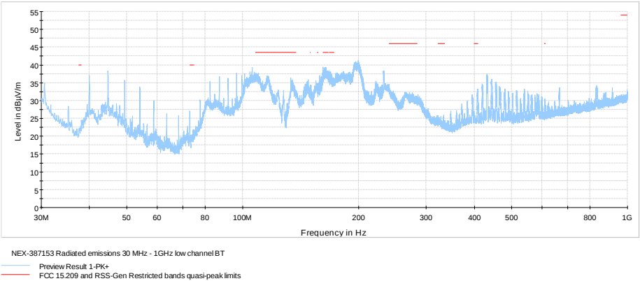
Figure 8.6-27: Radiated spurious emissions below 1 GHz, low channel
