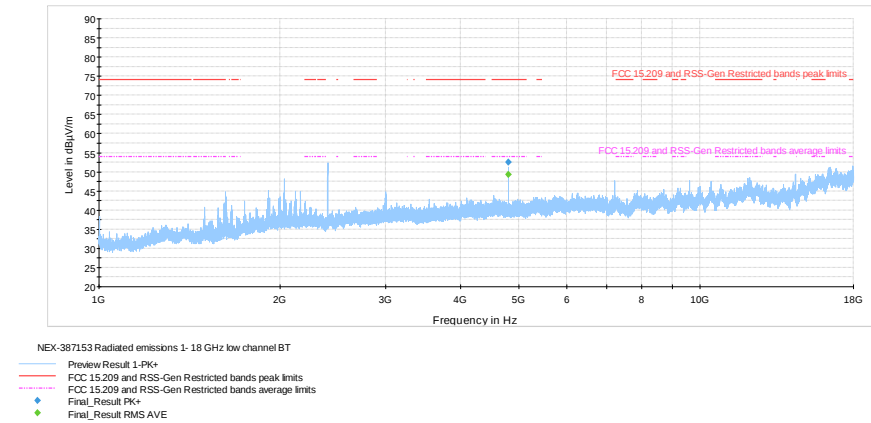
Figure 8.6-30: Radiated spurious emissions within 1-18 GHz, low channel
