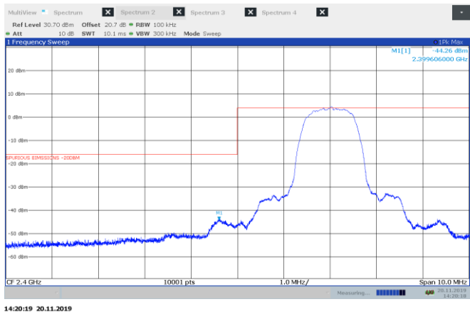
Figure 8.6-3: Conducted spurious emissions at the lower band edge for \pi/4 -DQPSK modulation, hopping off
