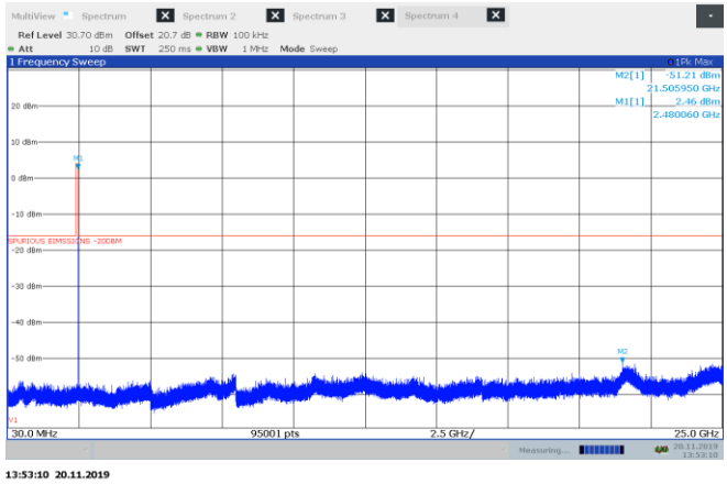
Figure 8.6-26: Conducted spurious emissions for BLE, high channel
