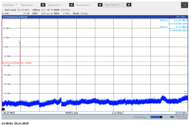
Figure 8.6-24: Conducted spurious emissions for BLE, low channel
