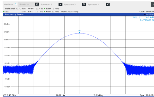
Figure 8.4-1: Output power sample plot
