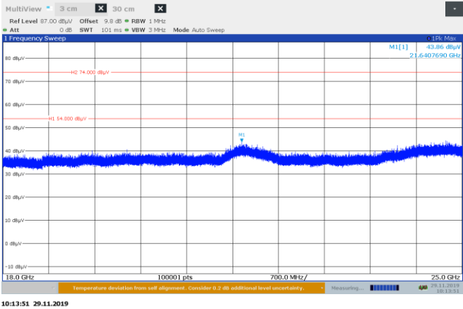
Figure 8.6-33: Radiated spurious emissions above 18 GHz, low channel
