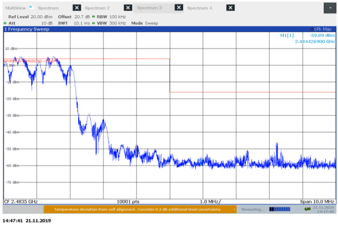
Figure 8.6-14: Conducted spurious emissions at the upper band edge for 8DPSK modulation, hopping on
