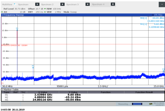
Figure 8.6-16: Conducted spurious emissions for GFSK, mid channel
