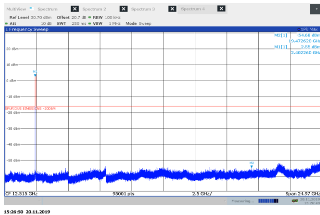
Figure 8.6-21: Conducted spurious emissions for 8DPSK, low channel
