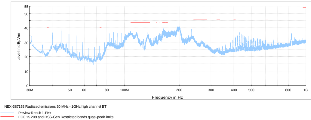
Figure 8.6-29: Radiated spurious emissions below 1 GHz, high channel
