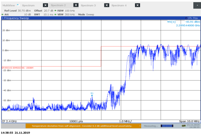
Figure 8.6-4: Conducted spurious emissions at the lower band edge for \pi/4 -DQPSK modulation, hopping on
