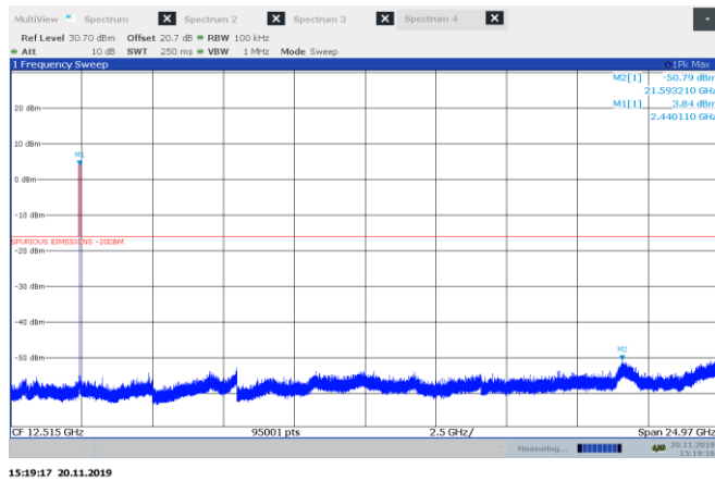
Figure 8.6-19: Conducted spurious emissions for \pi/4 -DQPSK, mid channel
