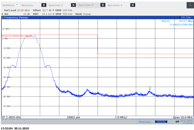
Figure 8.6-8: Conducted spurious emissions at the upper band edge for BLE modulation
