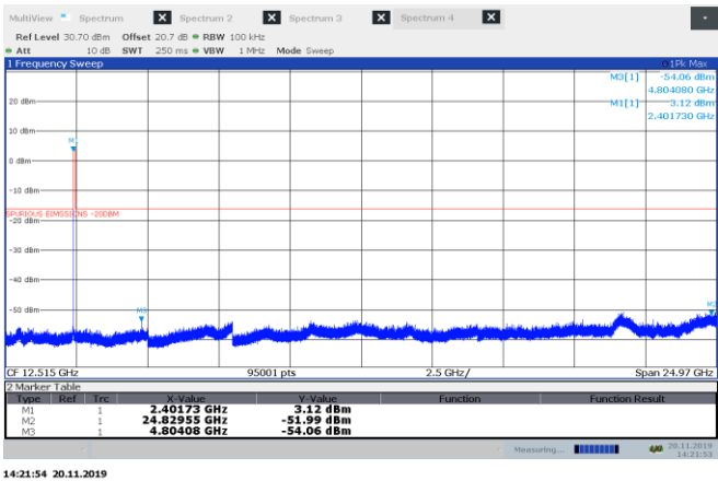
Figure 8.6-18: Conducted spurious emissions for \pi/4 -DQPSK, low channel
