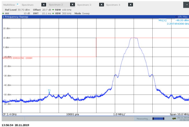
Figure 8.6-1: Conducted spurious emissions at the lower band edge for GFSK modulation, hopping off
