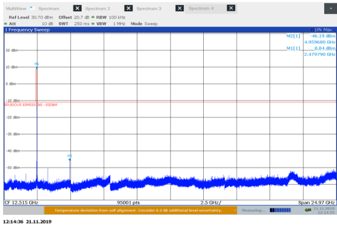
Figure 8.6-17: Conducted spurious emissions for GFSK, high channel
