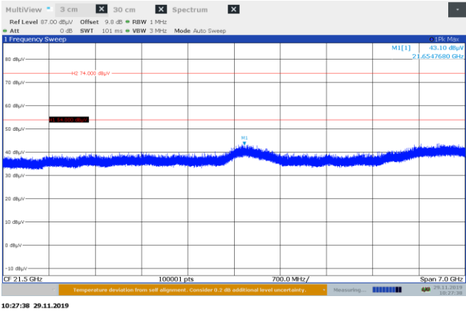
Figure 8.6-35: Radiated spurious emissions above 18 GHz, high channel
