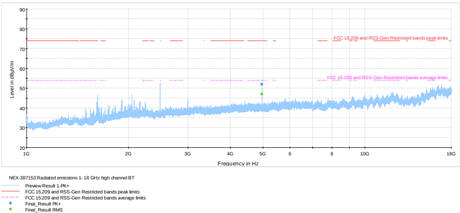
Figure 8.6-32: Radiated spurious emissions within 1-18 GHz, high channel
