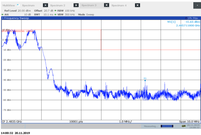
Figure 8.6-10: Conducted spurious emissions at the upper band edge for GFSK modulation, hopping on
