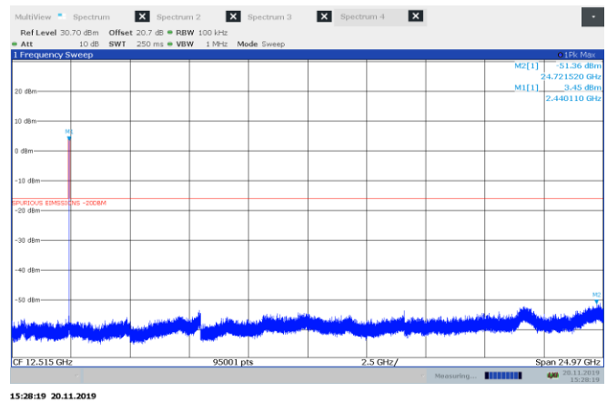
Figure 8.6-22: Conducted spurious emissions for 8DPSK, mid channel
