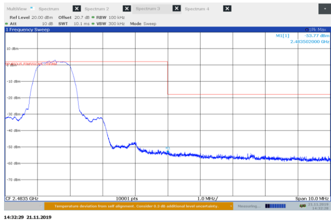
Figure 8.6-11: Conducted spurious emissions at the low upper band edge for \pi/4 -DQPSK modulation, hopping off
