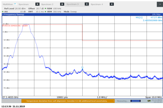
Figure 8.6-9: Conducted spurious emissions at the upper band edge for GFSK modulation, hopping off
