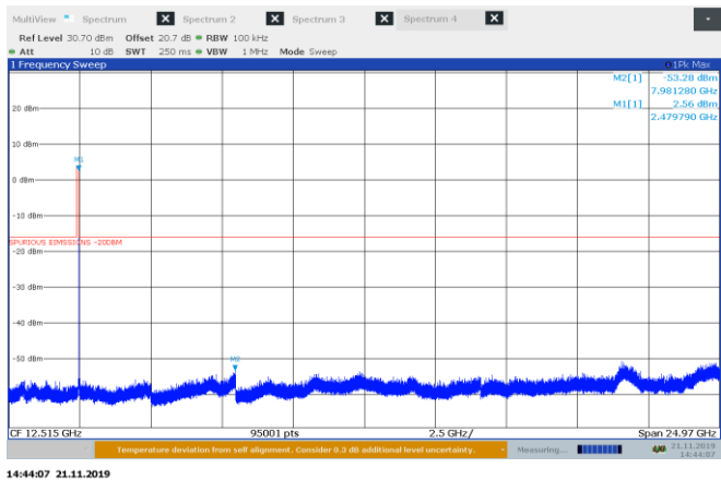
Figure 8.6-23: Conducted spurious emissions for 8DPSK, high channel
