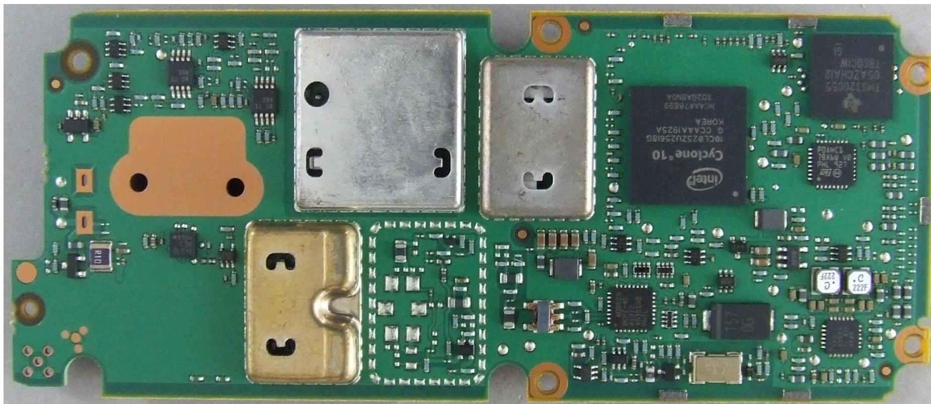
Photograph 03: Receive-Transmit PCB - bottom (with shields)
