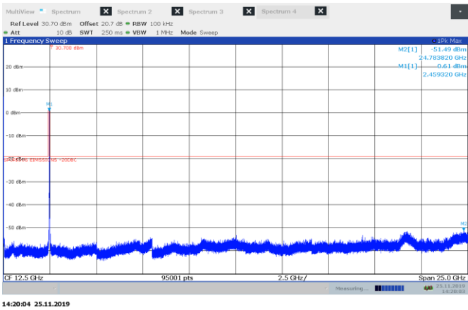
Figure 8.5-6: Conducted spurious emissions for 802.11 g, high channel
