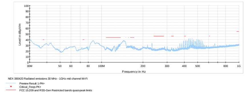
Figure 8.5-14: Radiated spurious emissions below 1 GHz, mid channel
