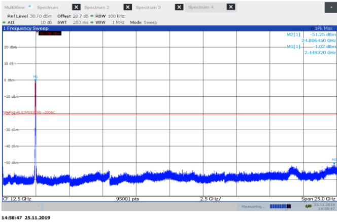
Figure 8.5-12: Conducted spurious emissions for 802.11n 40high channel
