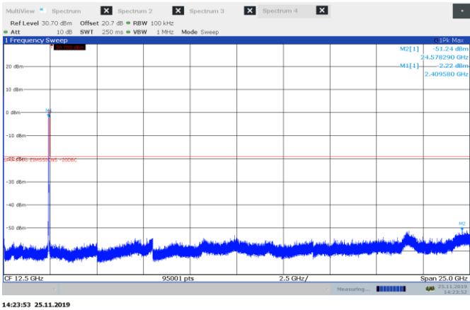
Figure 8.5-4: Conducted spurious emissions for 802.11 g, low channel
