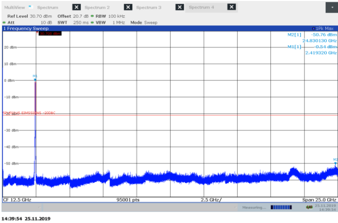
Figure 8.5-10: Conducted spurious emissions for 802.11n 40, low channel
