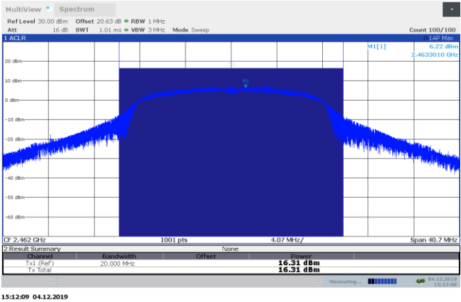
Figure 8.4-2: Conducted output power on 802.11g, sample plot
