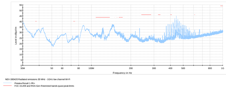
Figure 8.5-13: Radiated spurious emissions below 1 GHz, low channel
