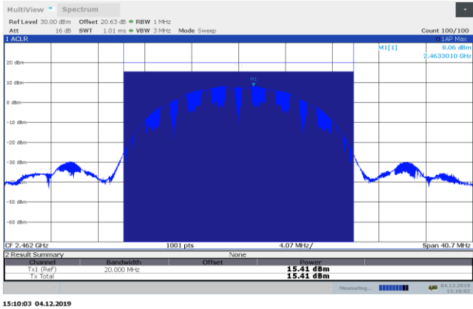
Figure 8.4-1: Conducted output power 802.11b, sample plot
