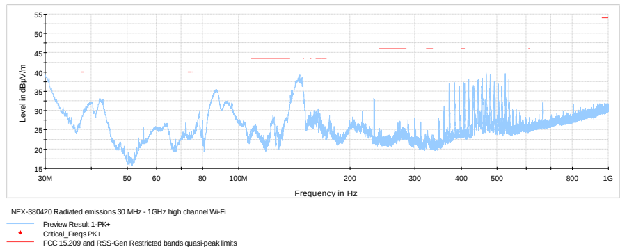
Figure 8.5-15: Radiated spurious emissions below 1 GHz, high channel
