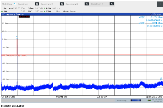
Figure 8.5-8: Conducted spurious emissions for 802.11n 20, mid channel
