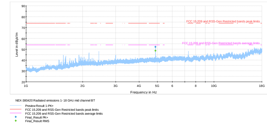
Figure 8.6-31: Radiated spurious emissions within 1–18 GHz, mid channel
