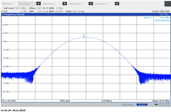
Figure 8.5-1: Output power sample plot
