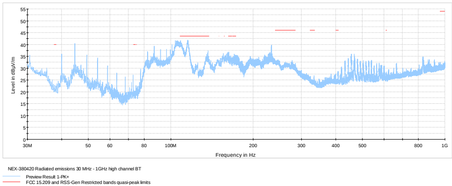
Figure 8.6-29: Radiated spurious emissions below 1 GHz, high channel
