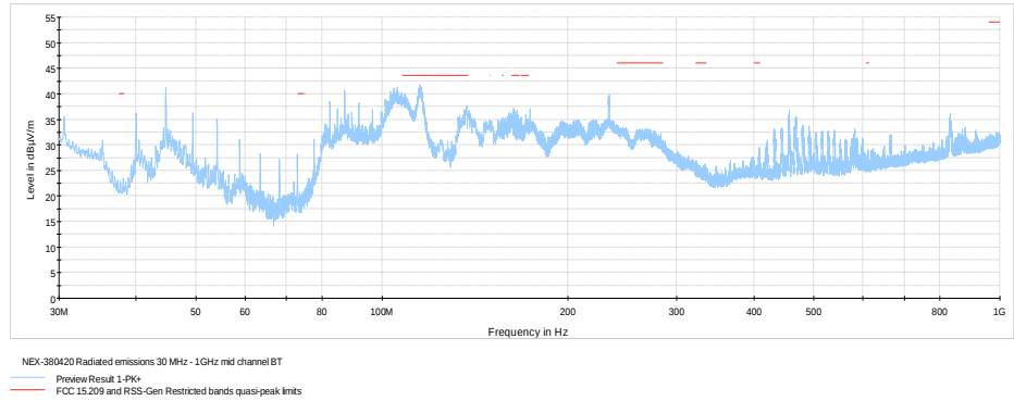
Figure 8.6-28: Radiated spurious emissions below 1 GHz, mid channel
