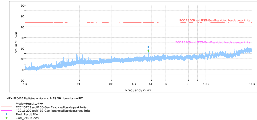
Figure 8.6-30: Radiated spurious emissions within 1–18 GHz, low channel
