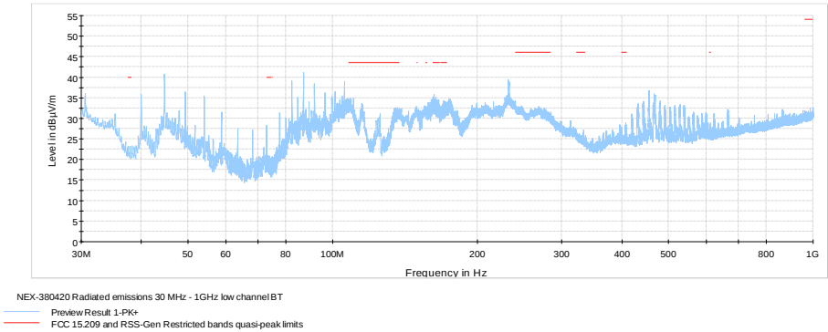
Figure 8.6-27: Radiated spurious emissions below 1 GHz, low channel
