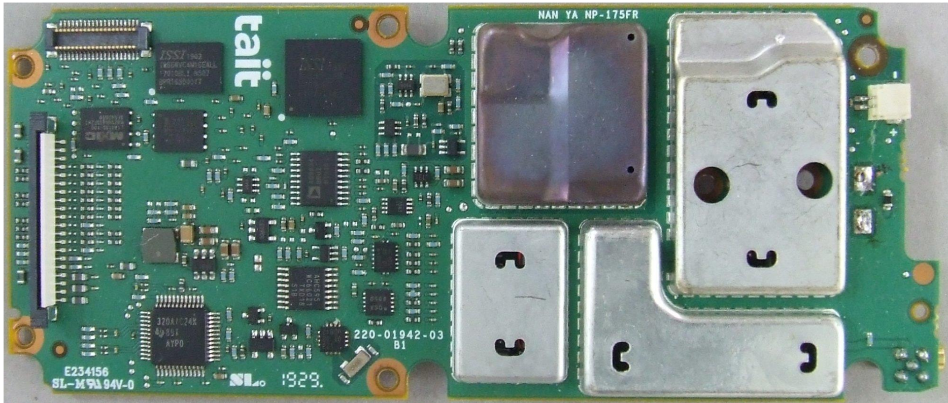
Photograph 01: Receive-Transmit PCB – top (with shields)
