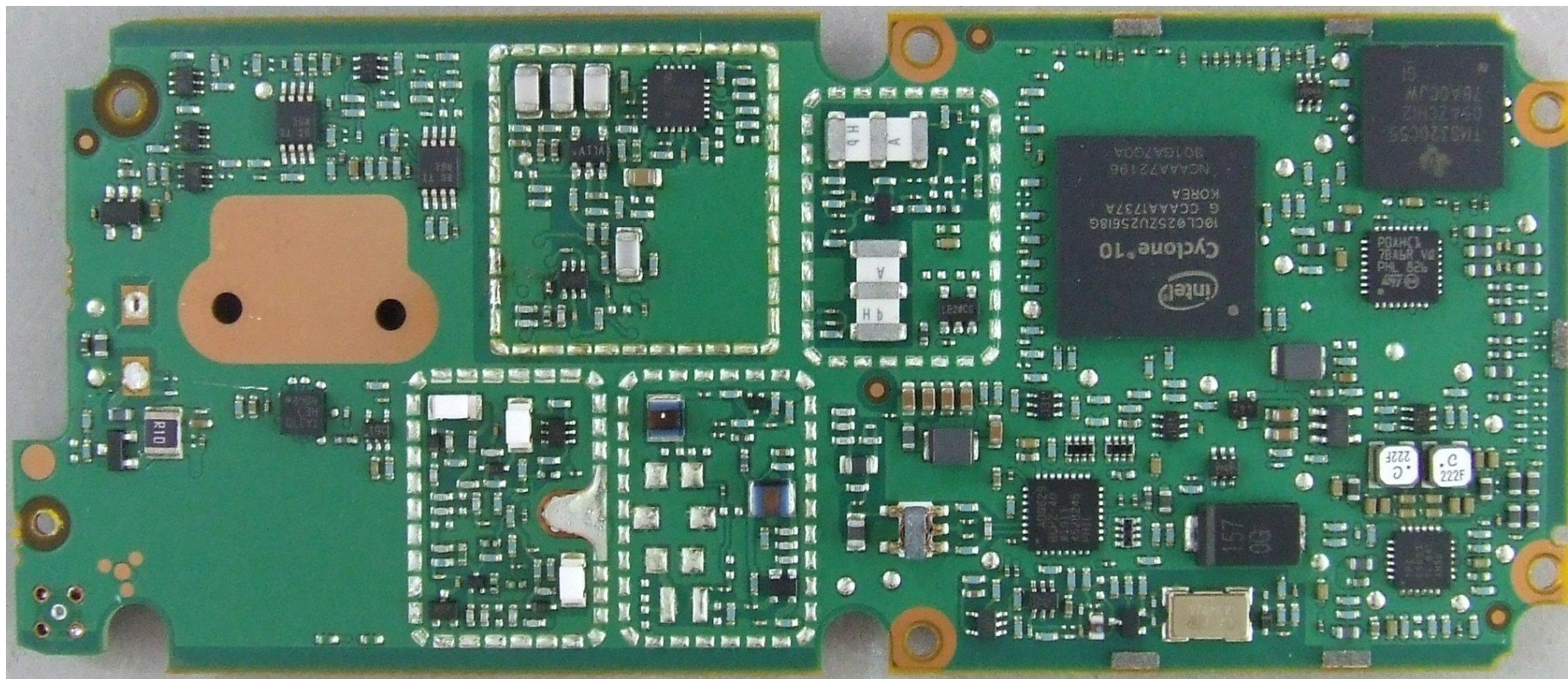
Photograph 04: Receive-Transmit PCB - bottom (without shields)
