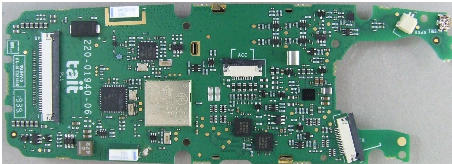
Photograph 06: Control PCB - Bottom
