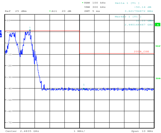
Figure 8.6-8: Conducted spurious emissions at the upper band edge for BLE modulation
