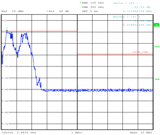
Figure 8.6-12: Conducted spurious emissions at the upper band edge for \pi/4 -DQPSK modulation, hopping on
