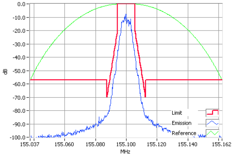
P25II 155.1000MHz Mask D 5W RBW=100Hz, VBW=1000Hz, Detector Mode=Peak Result=Pass
