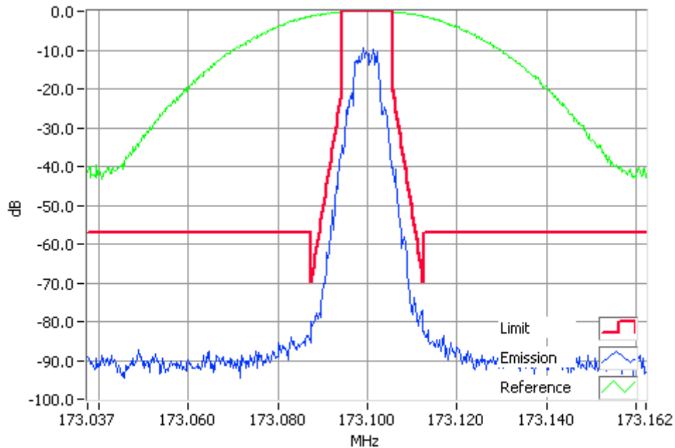
DMR 173.1000MHz Mask D 5W RBW=100Hz, VBW=1000Hz, Detector Mode=Peak Result=Pass
