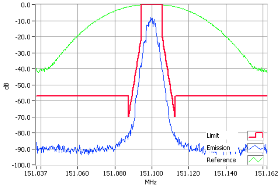
DMR 151.1000MHz Mask D 5W RBW=100Hz, VBW=1000Hz, Detector Mode=Peak Result=Pass
