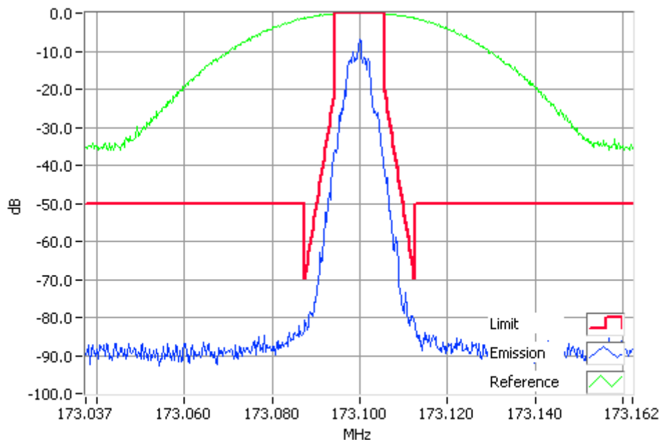
DMR 173.1000MHz Mask D 1W RBW=100Hz, VBW=1000Hz, Detector Mode=Peak Result=Pass
