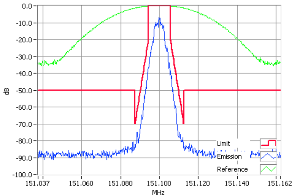
DMR 151.1000MHz Mask D 1W RBW=100Hz, VBW=1000Hz, Detector Mode=Peak Result=Pass
