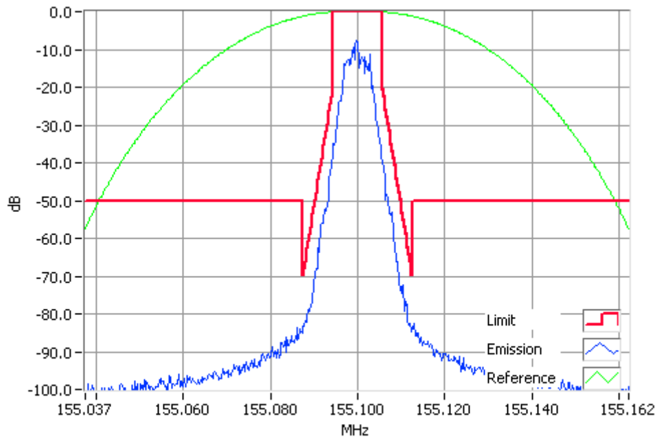
P25II 155.1000MHz Mask D 1W RBW=100Hz, VBW=1000Hz, Detector Mode=Peak Result=Pass
