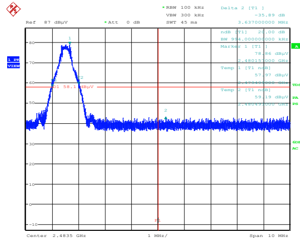
Figure 8.2-12: Radiated spurious band edge emission at 2.4835 GHz, QPSK modulation, 20 dBc limit
