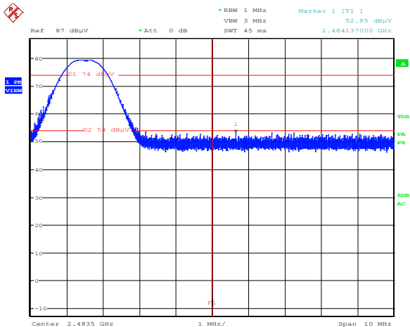
Figure 8.2-11: Radiated spurious band edge emission at 2.4835 GHz, QPSK modulation, 15.209 limits
