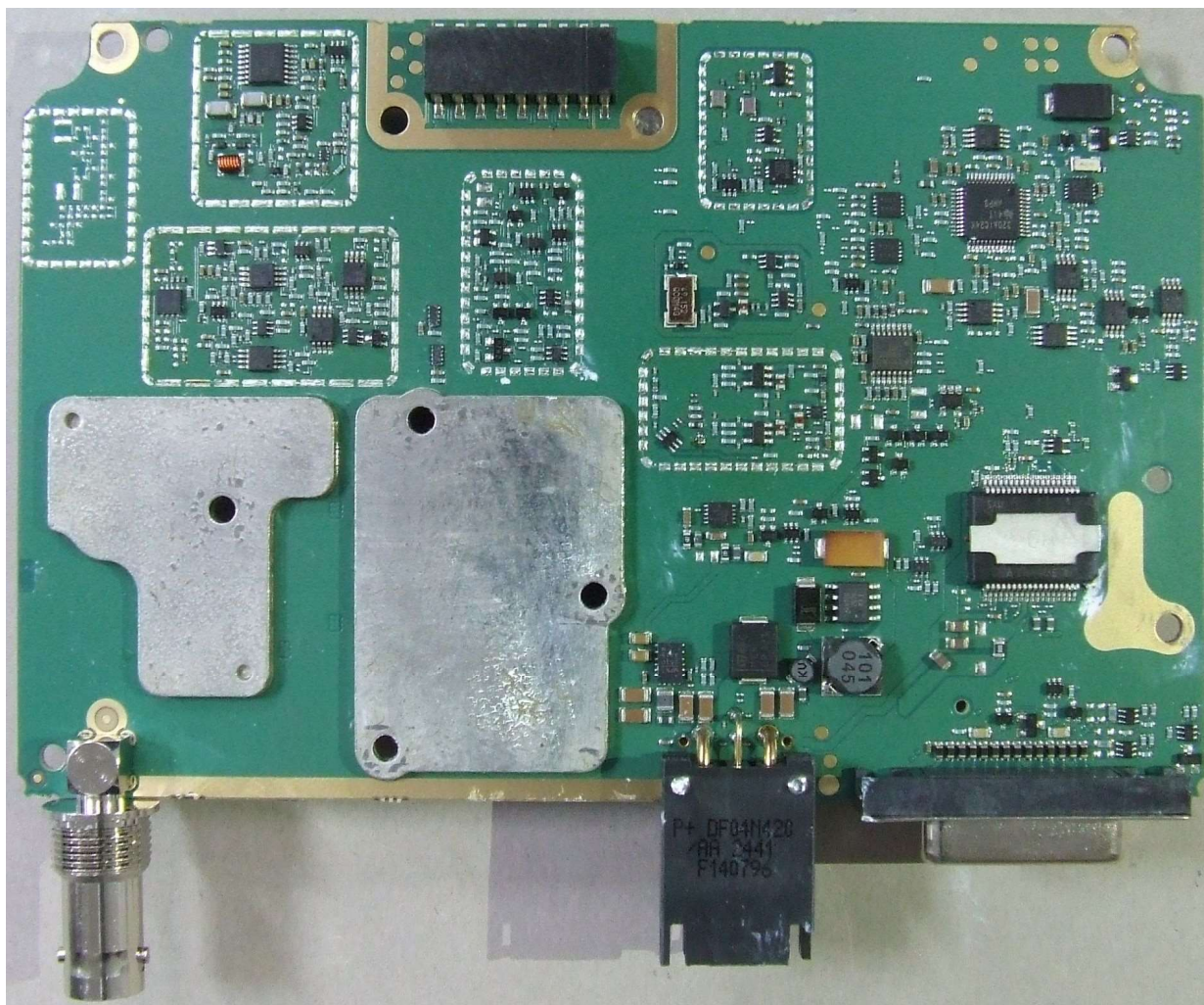
Photograph 4: Radio PCB bottom without shields
