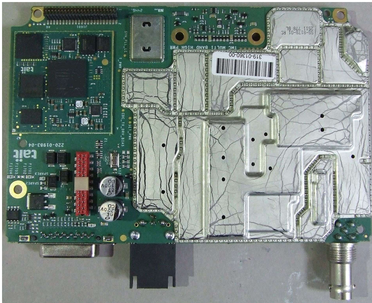
Photograph 1: Radio PCB top with shields
