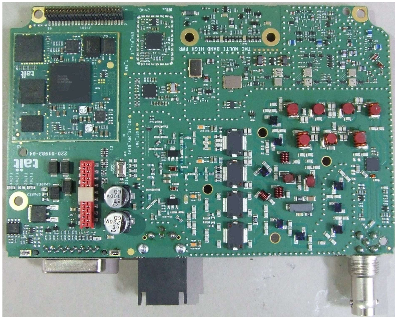
Photograph 2: Radio PCB top without shields
