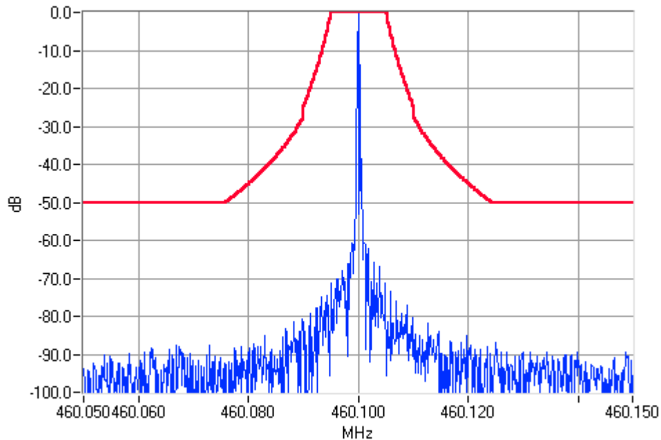
Unmodulated 460.1000MHz Mask C 1W Pass
