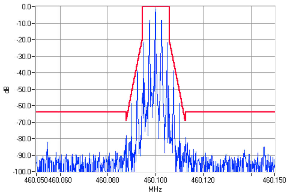
Analogue Modulation 460.1000MHz Mask D 25W Pass
