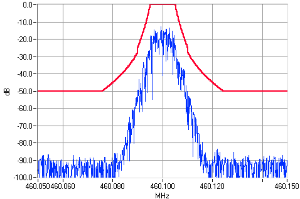
Digital Modulation 460.1000MHz Mask C 1W Pass
