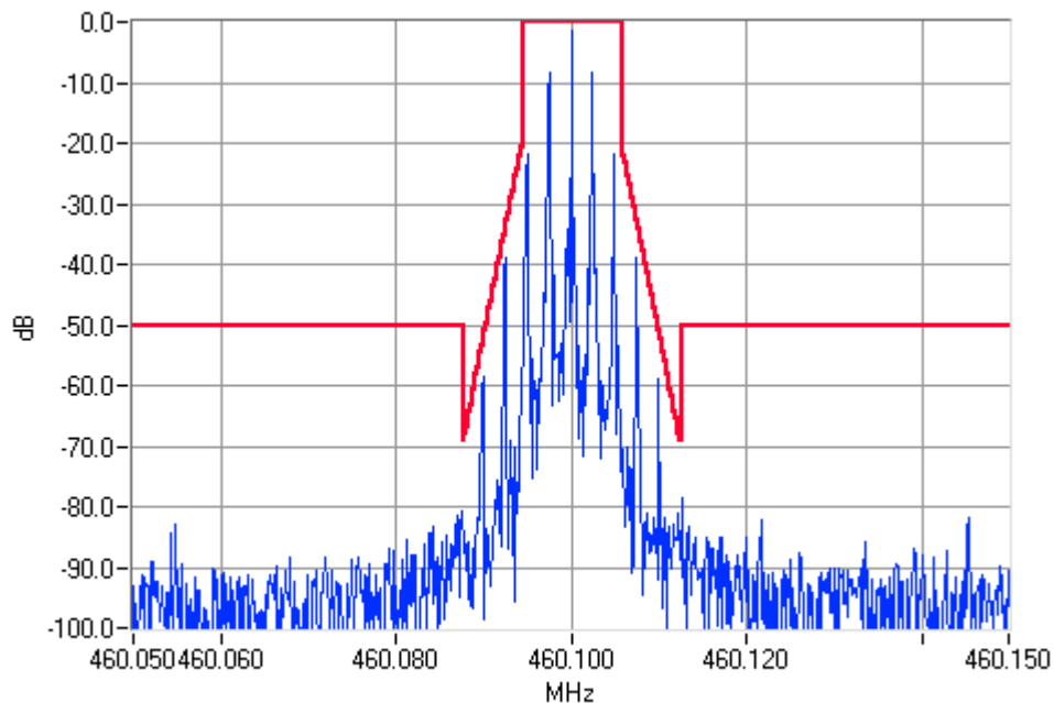
Analogue Modulation 460.1000MHz Mask D 1W Pass
