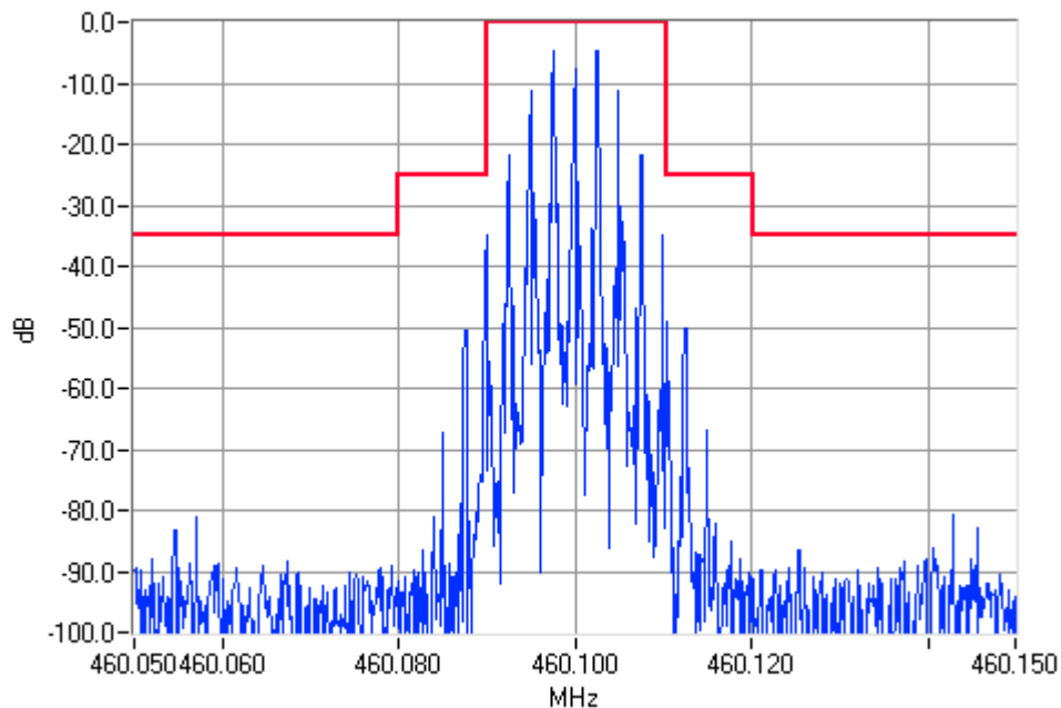
Analogue Modulation 460.1000MHz Mask B 25W Pass
