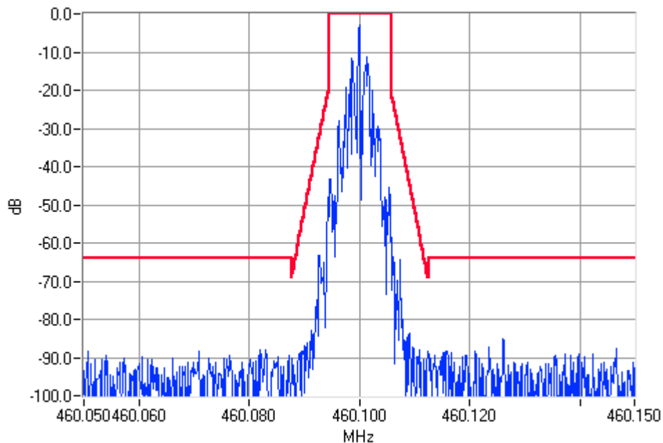
Digital Modulation 460.1000MHz Mask D 25W Pass
