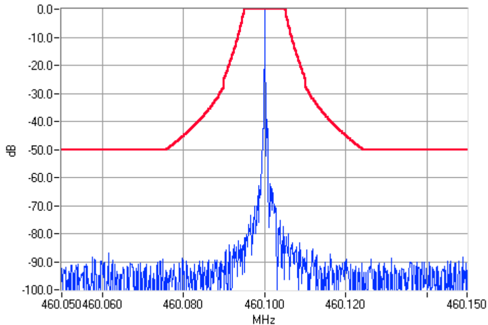
Unmodulated 460.1000MHz Mask C 25W Pass
