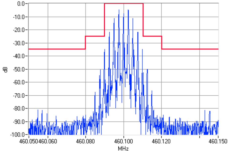
Analogue Modulation 460.1000MHz Mask B 1W Pass
