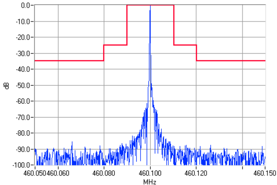
Unmodulated 460.1000MHz Mask B 25W Pass
