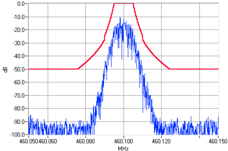
Digital Modulation 460.1000MHz Mask C 25W Pass
