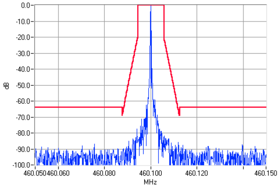
Unmodulated 460.1000MHz Mask D 25W Pass
