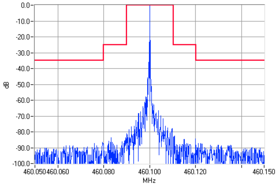
Unmodulated 460.1000MHz Mask B 1W Pass
