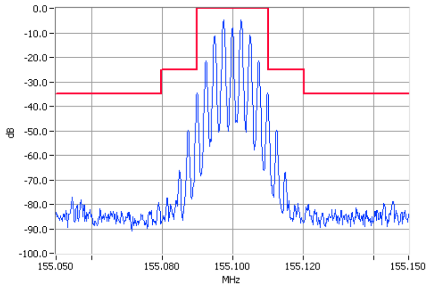
Analogue Modulation 155.1000MHz Mask B 50W Pass
