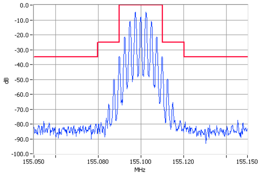
Analogue Modulation 155.1000MHz Mask B 10W Pass
