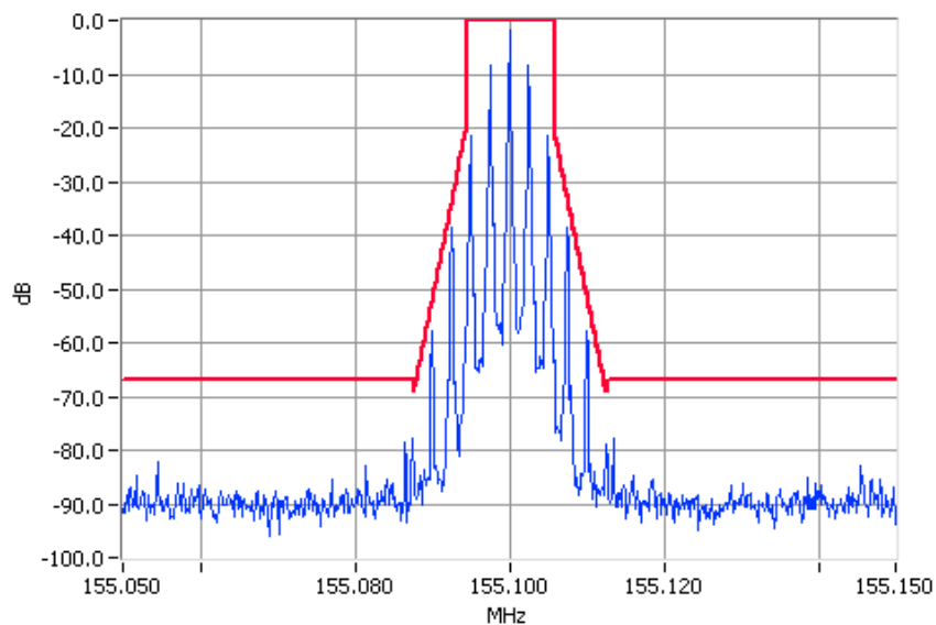
Analogue Modulation 155.1000MHz Mask D 50W Pass
