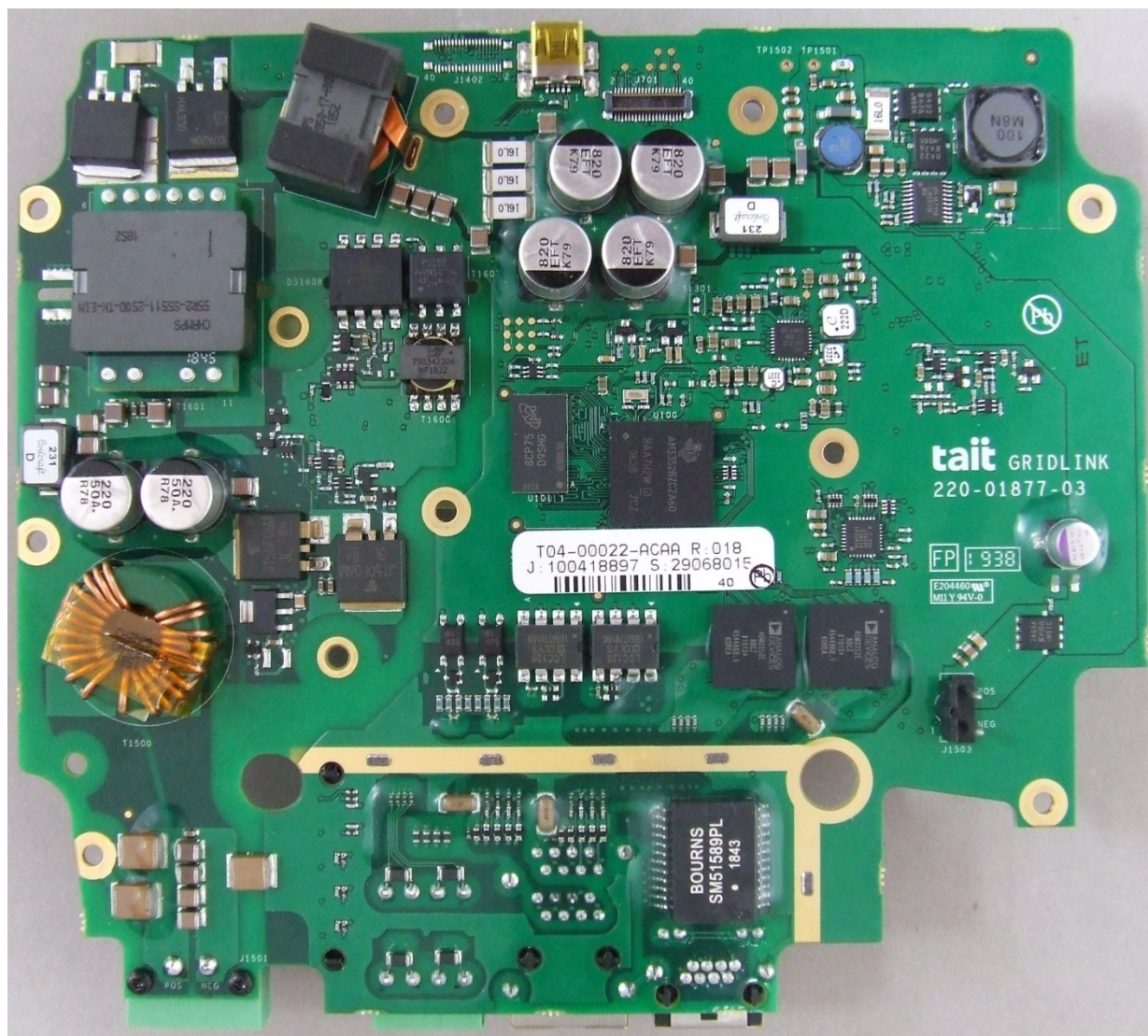
Photograph 01: Gridlink PCB top
