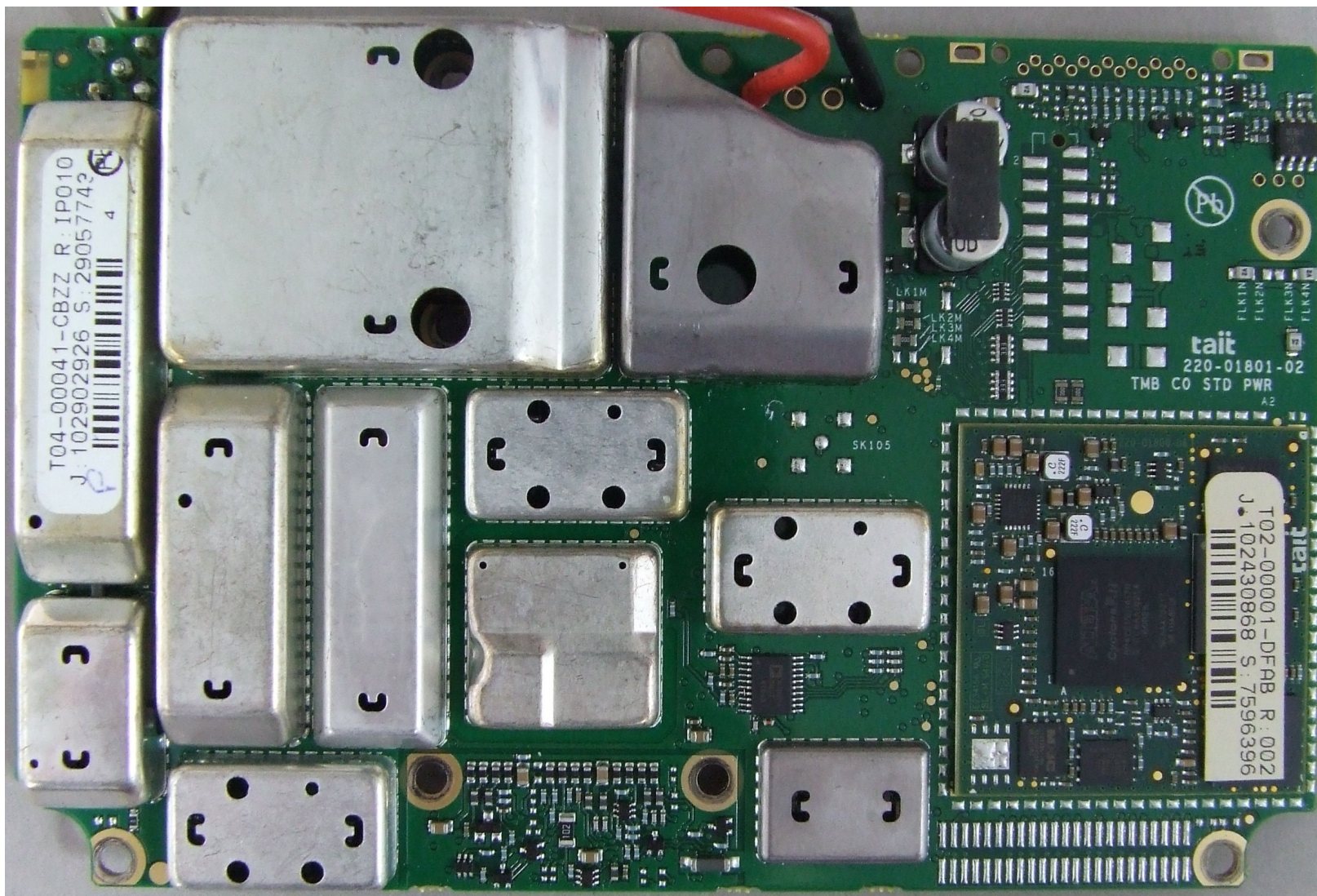
Photograph 03: RF PCB top with shields
