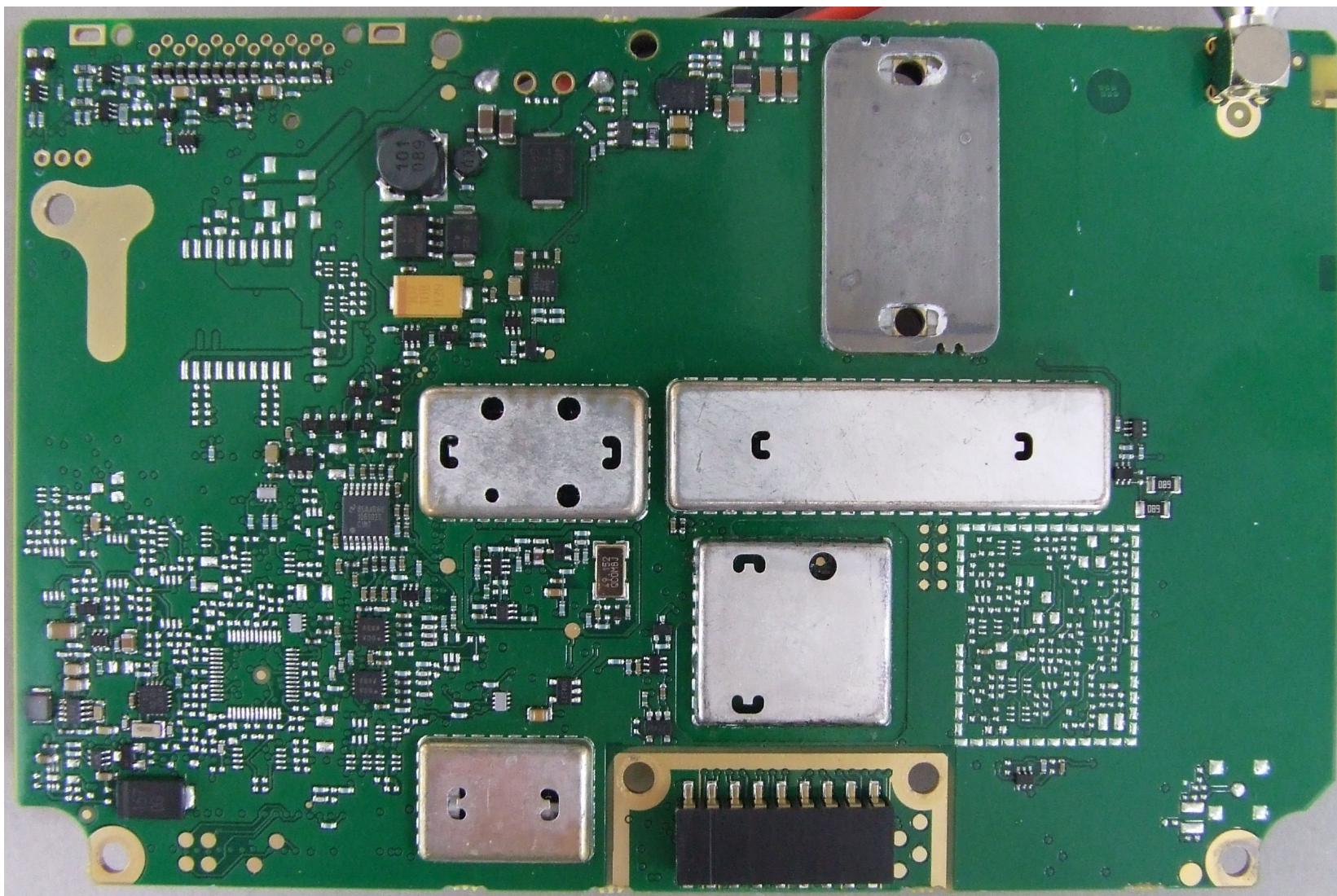
Photograph 05: RF PCB bottom with shields
