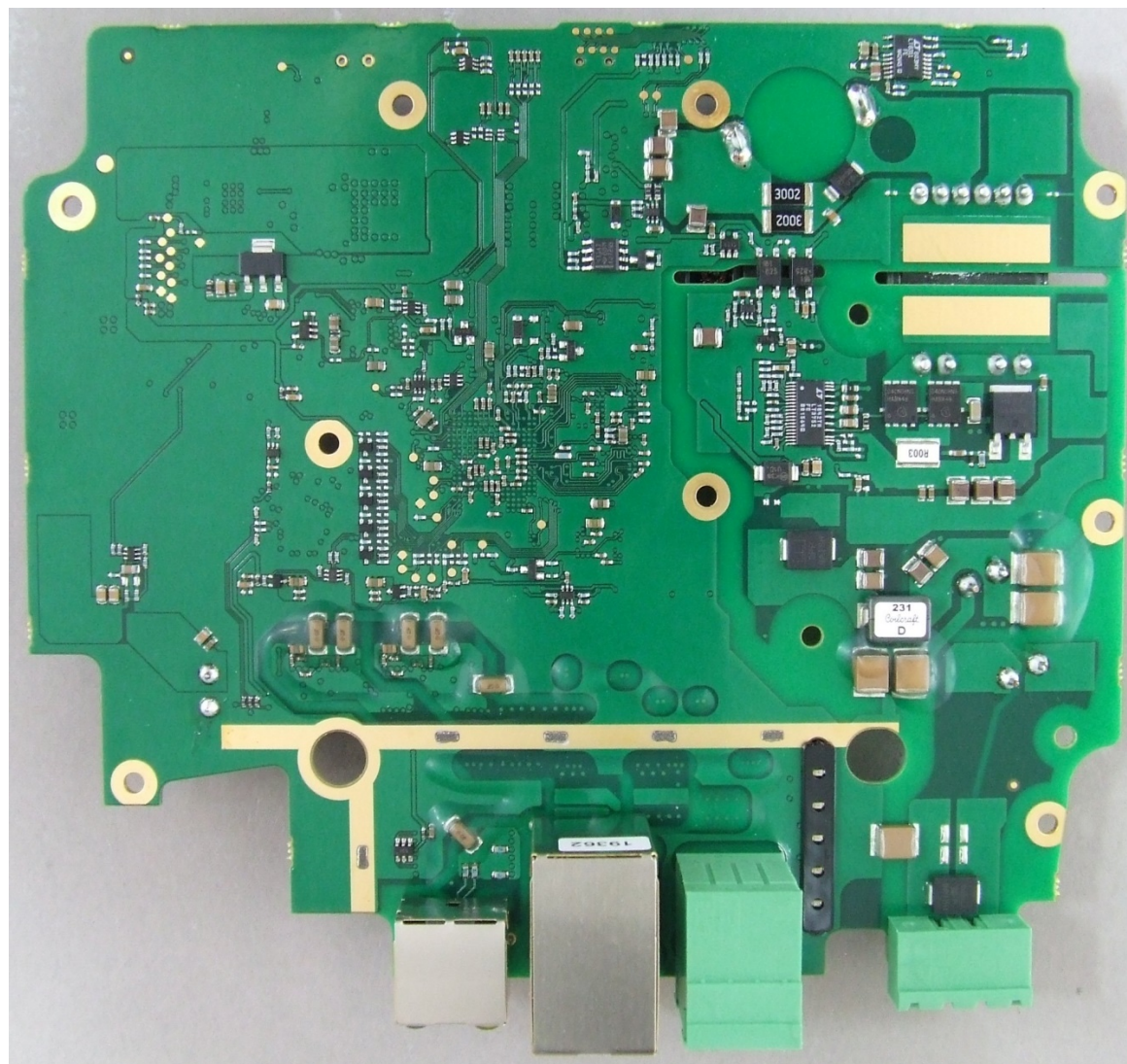
Photograph 02: Gridlink PCB bottom
