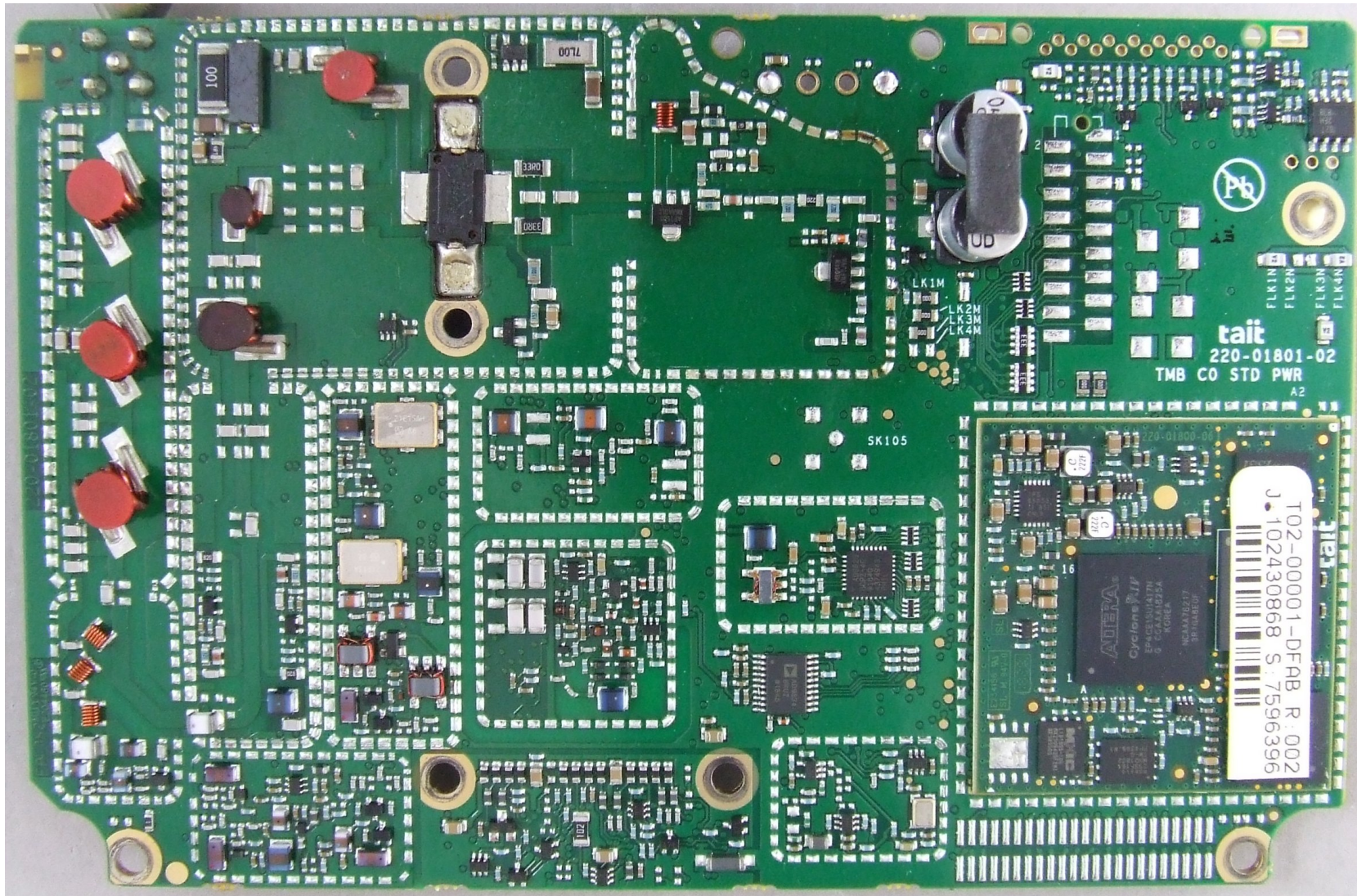
Photograph 04: RF PCB top without shields
