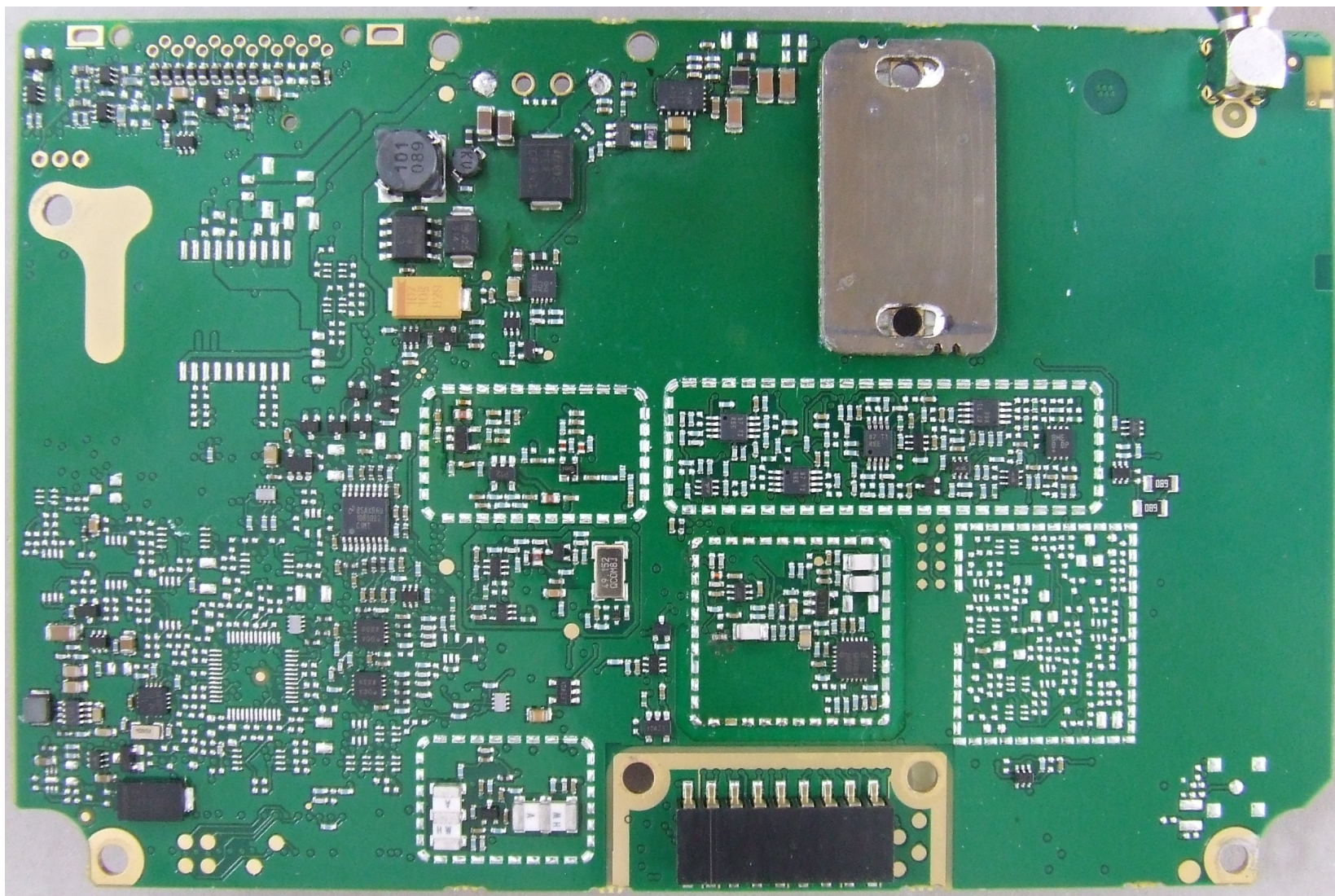
Photograph 06: RF PCB bottom without shields
