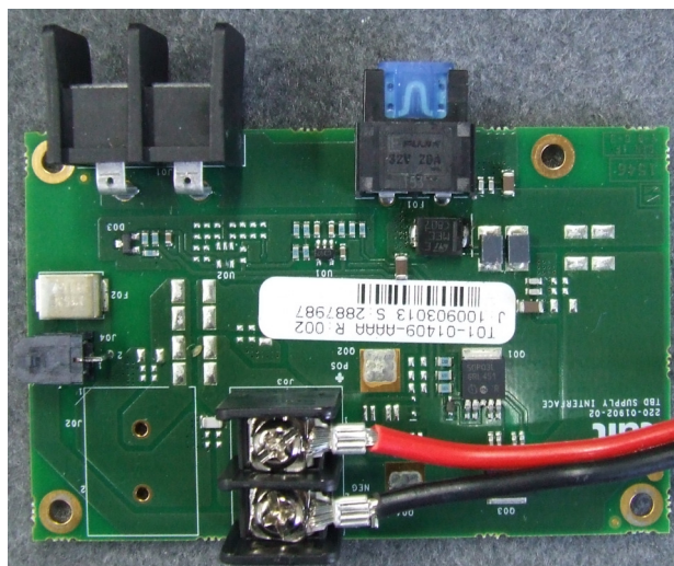
Photograph 05: Supply Interface PCB - Top
