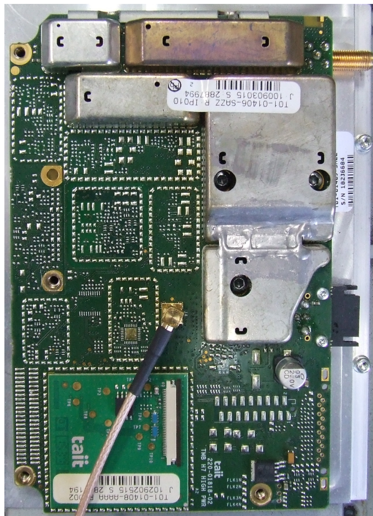
Photograph 07: Power Amplifier PCB – Top
