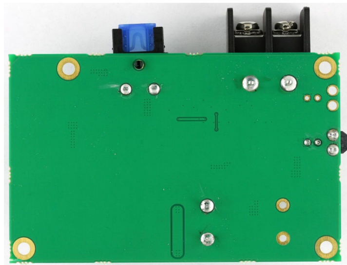
Photograph 06: Supply Interface PCB - Bottom
