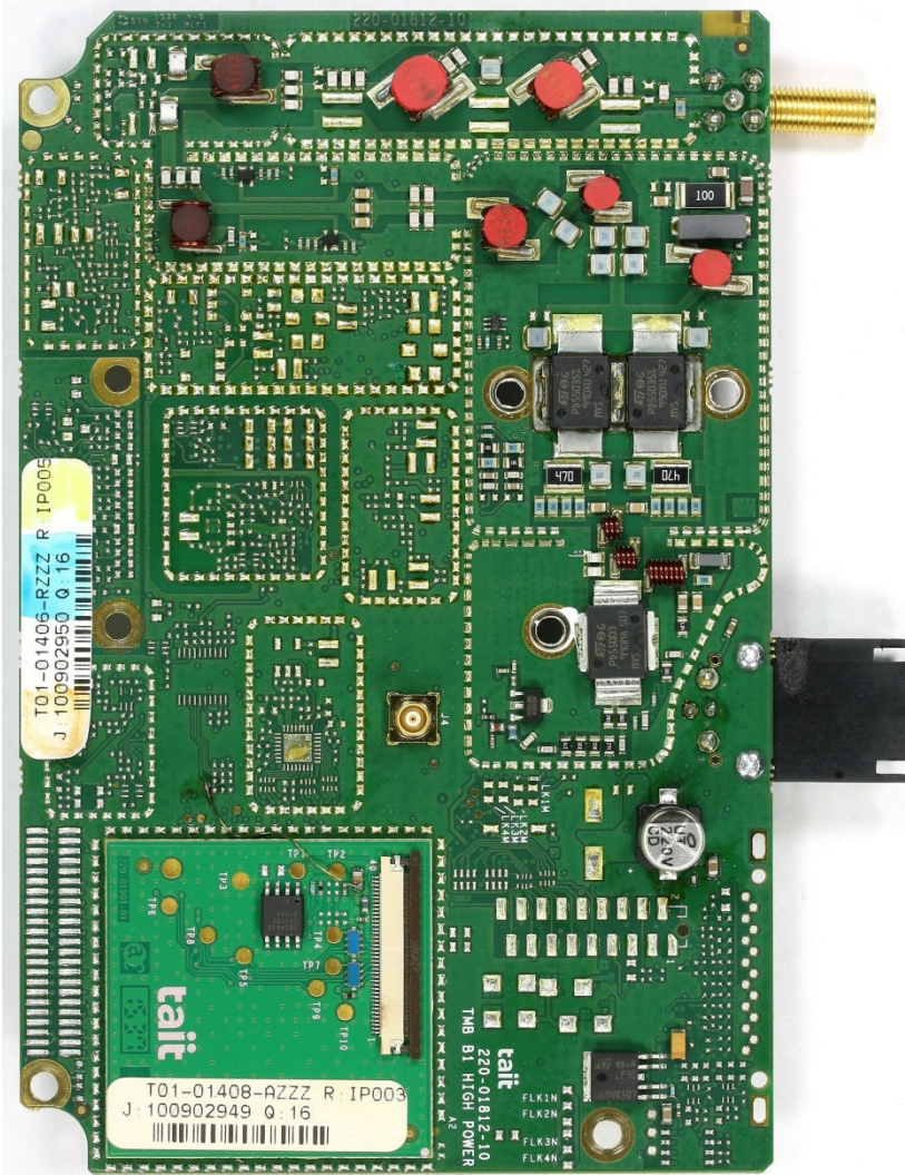
Photograph 08: Power Amplifier PCB – Top, cans off
