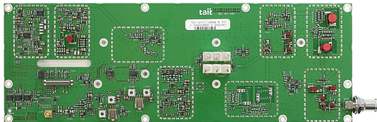
Photograph 14: Receiver Board (RXB) – Top (cans off)
