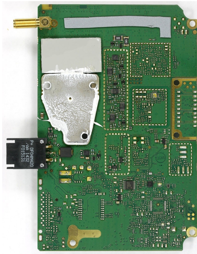
Photograph 09: Power Amplifier PCB – Bottom
