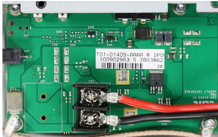
Photograph 05: Supply Interface PCB - Top
