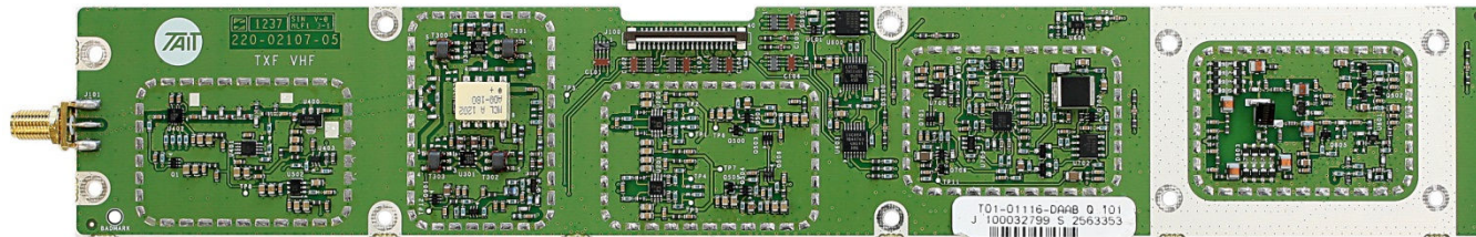
Photograph 17: Transmit Forward Power Board (TXF) – Top (cans off)
