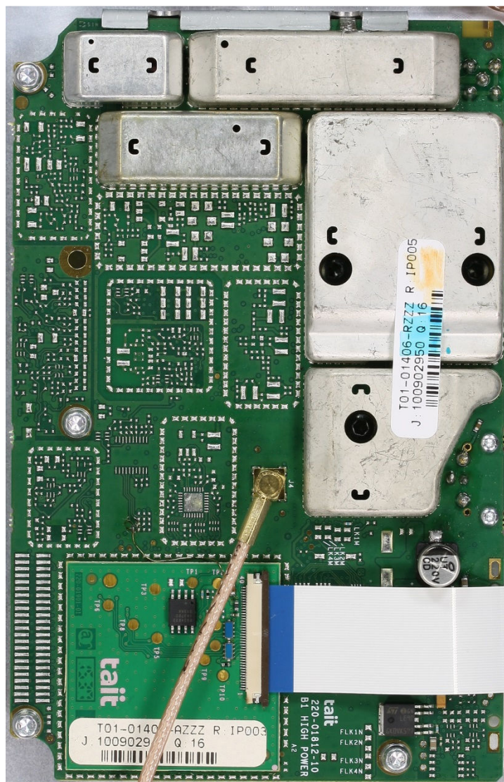
Photograph 07: Power Amplifier PCB – Top
