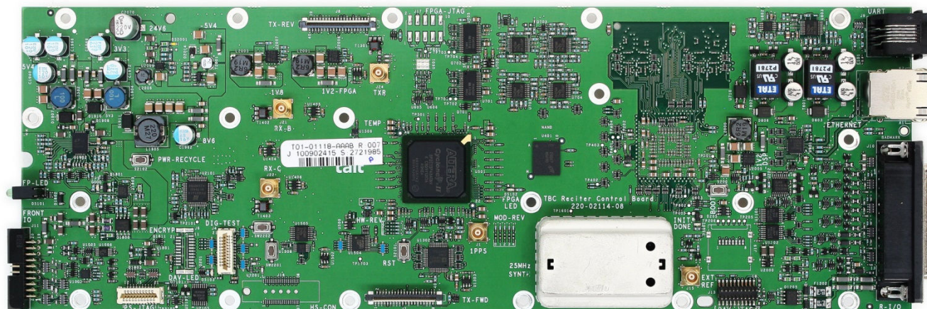
Photograph 10: Reciter Control Board (RCB) – Top
