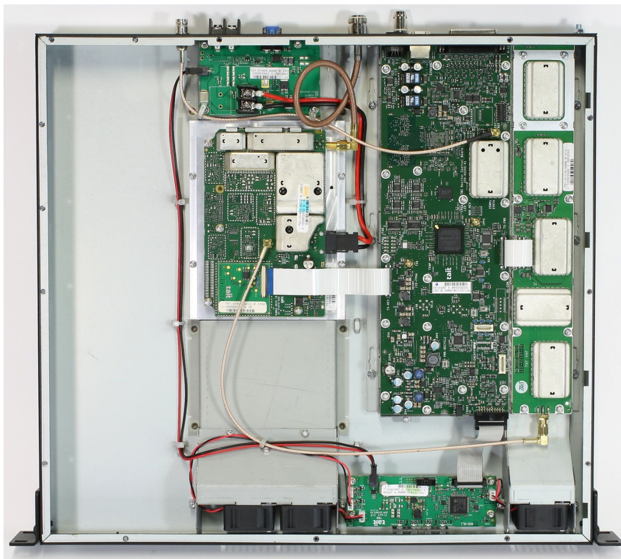
Photograph 01: Internal view
