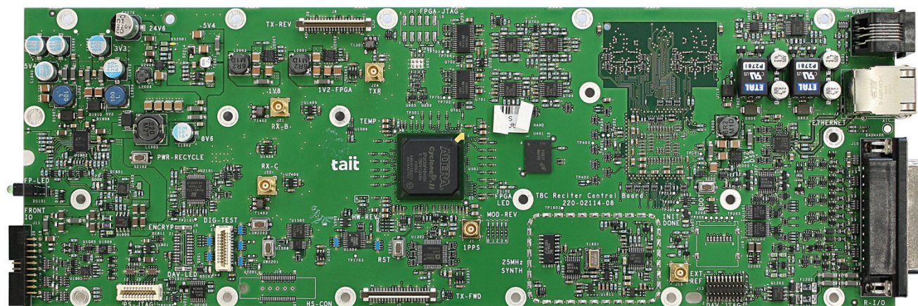
Photograph 11: Reciter Control Board (RCB) – Top (can off)
