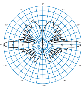
COL809-82 - E Plane
