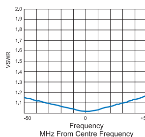
Typical VSWR response (ISM5803)
