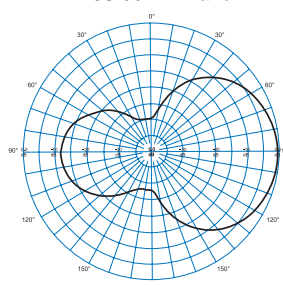
YB03-99 - E Plane
