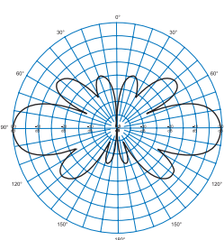
COL5806 - E Plane
