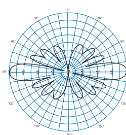
COL5808 - E Plane
