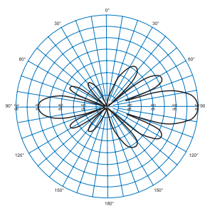
OA40-67 - E Plane
