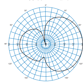
YB03-99 - H Plane
