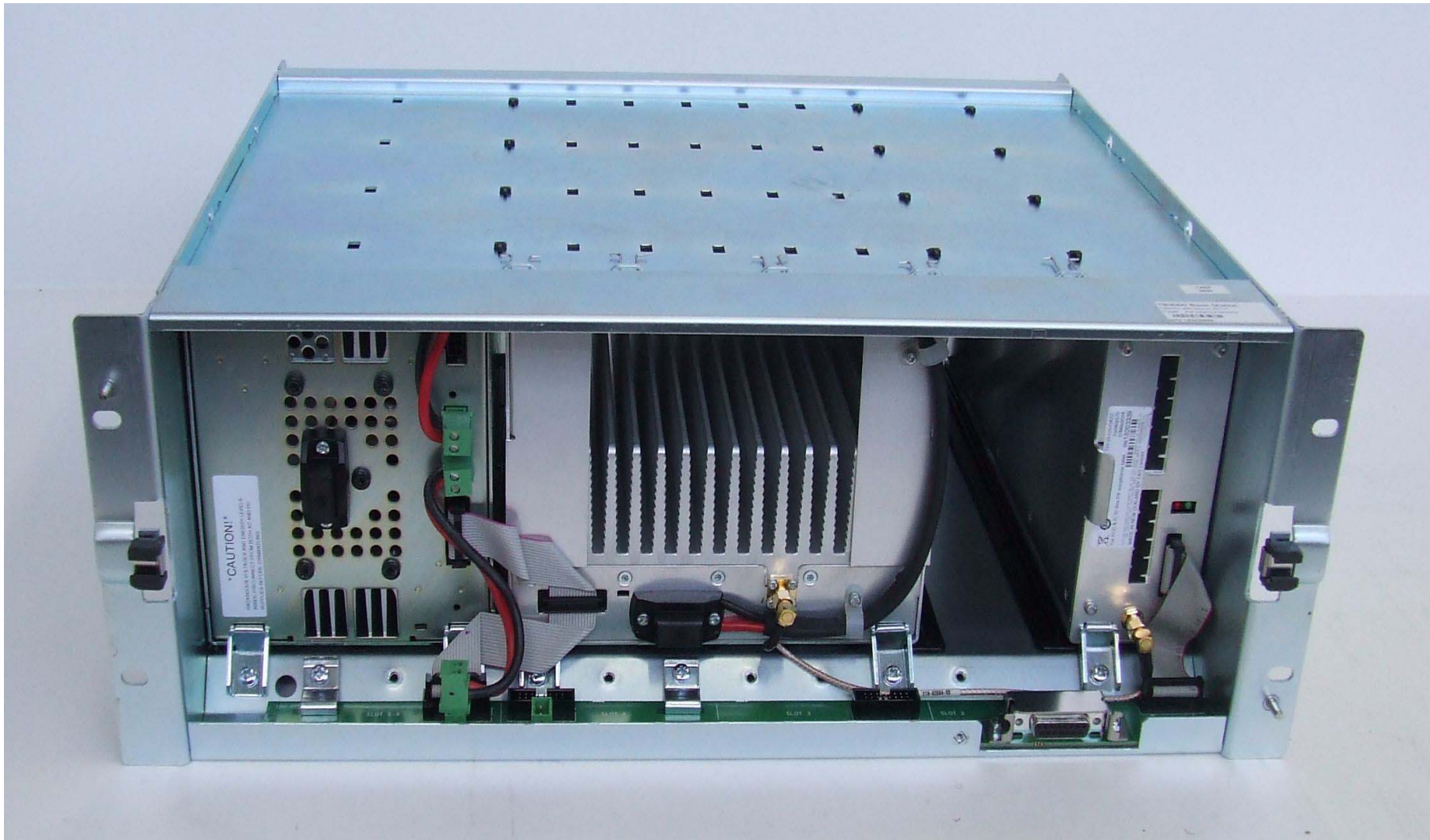
Photograph 04: 100W System – Internal view
