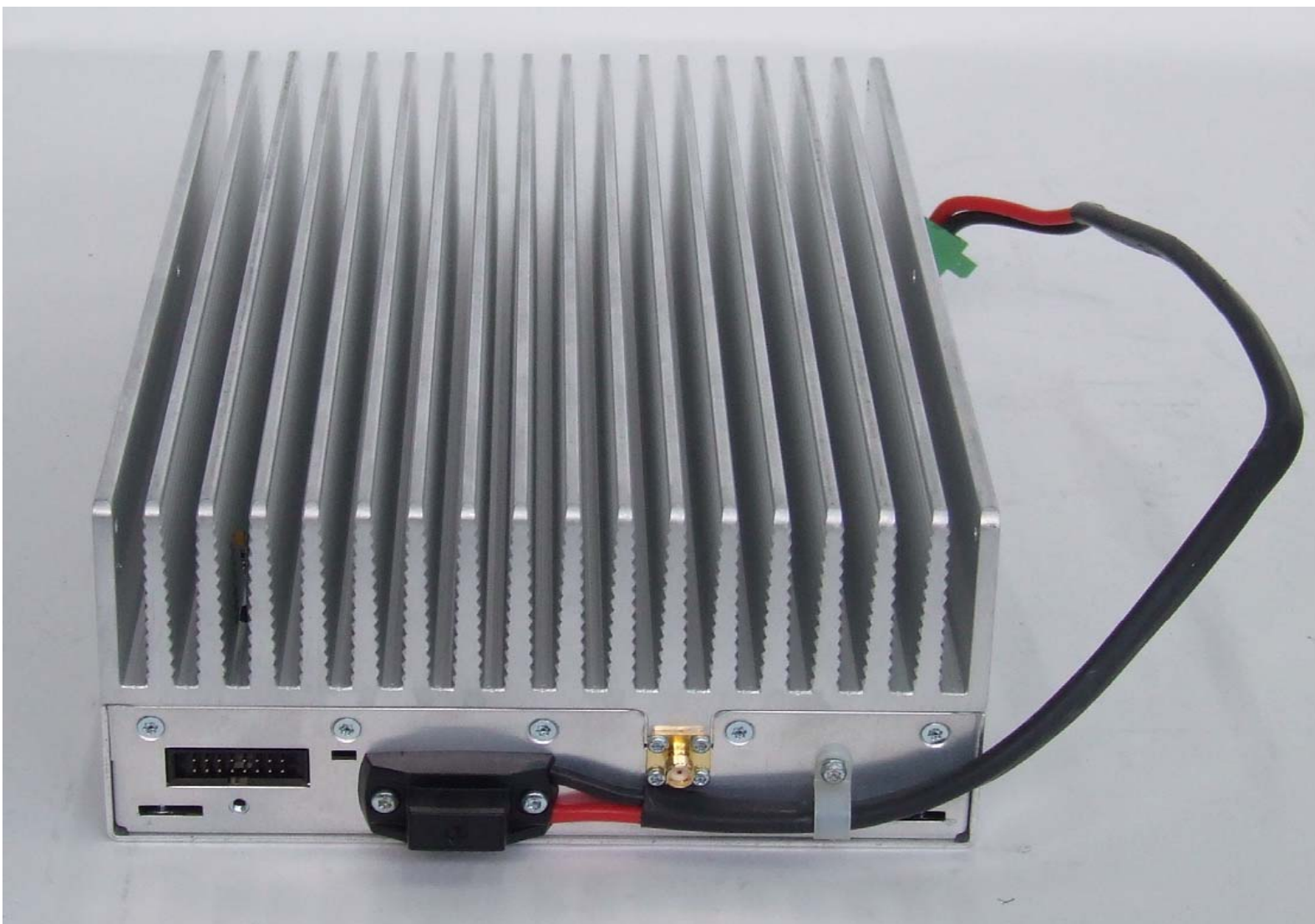
Photograph 06: 100W PA module – Front panel
