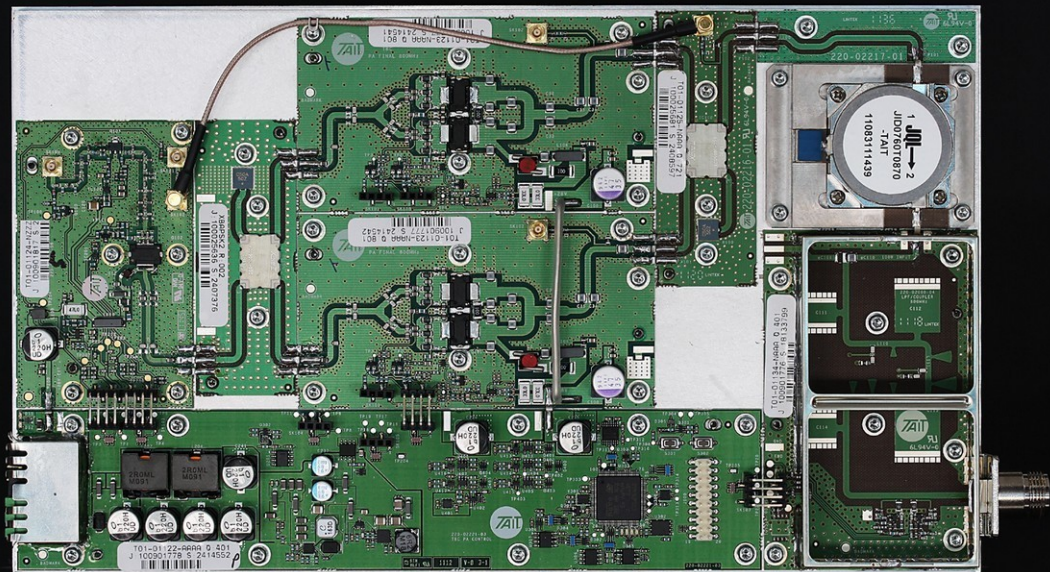
PA Layout With Cans Removed
