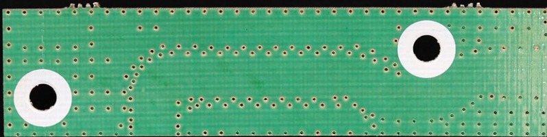
PA Circulator Board Bottom View
