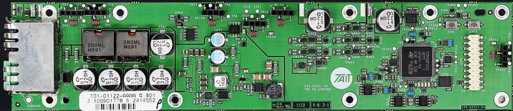
PA Control Board Top View
