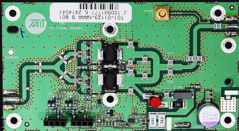
PA Final Board Top View
