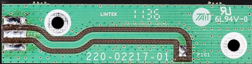
PA Circulator Board Top View
