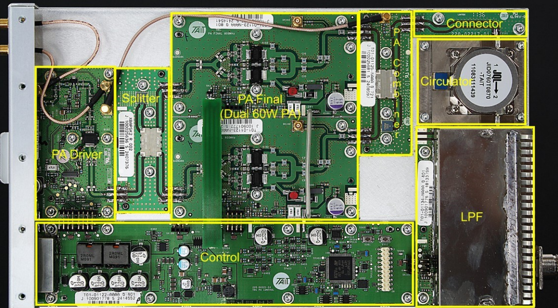
PA Annotated Layout Cans On
