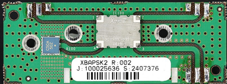
PA Splitter Board Top View
