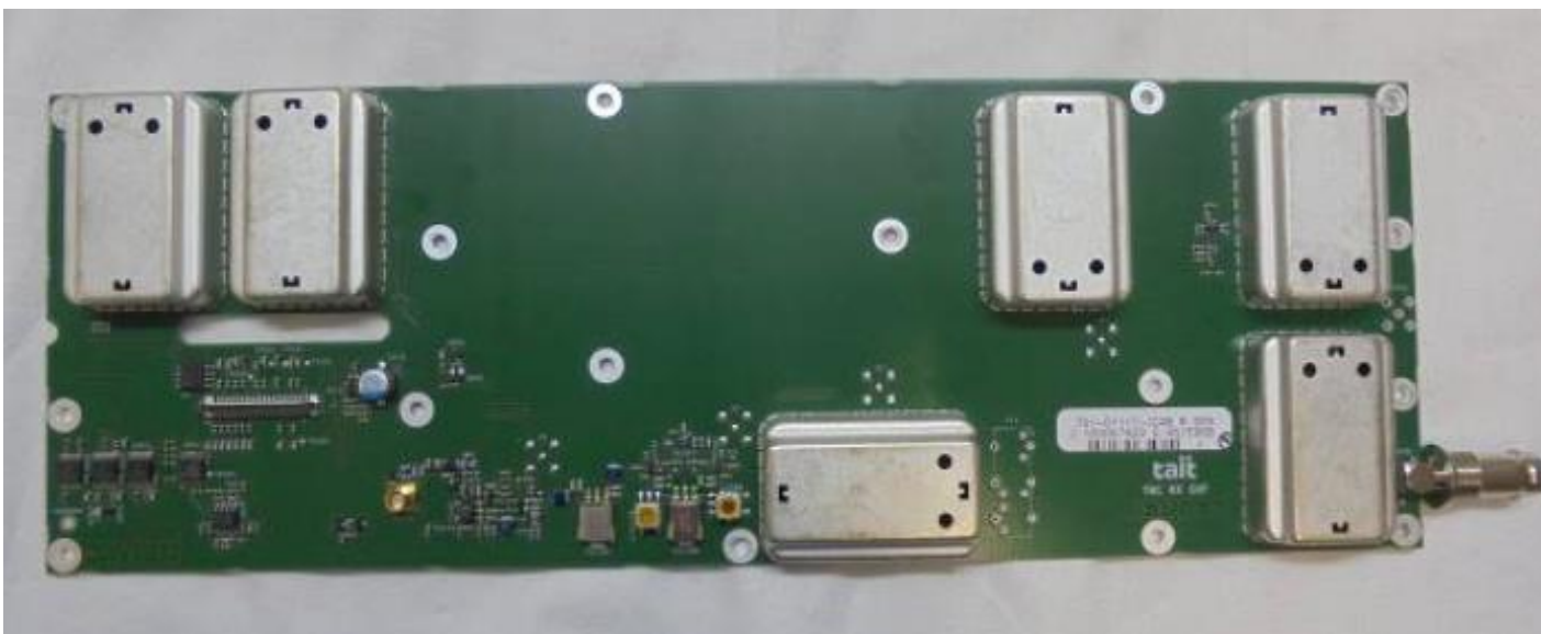
Photograph 03: Reciter Receiver PCB – Top (with shields)
