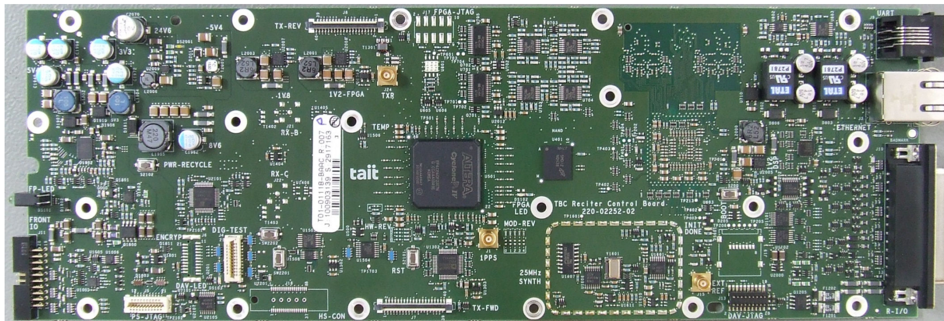
Photograph 07: Reciter Control PCB – Top (without shields)
