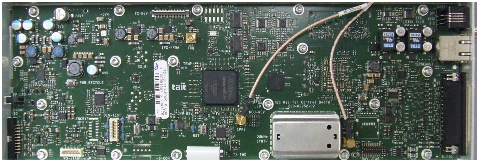
Photograph 06: Reciter Control PCB – Top (with shields)
