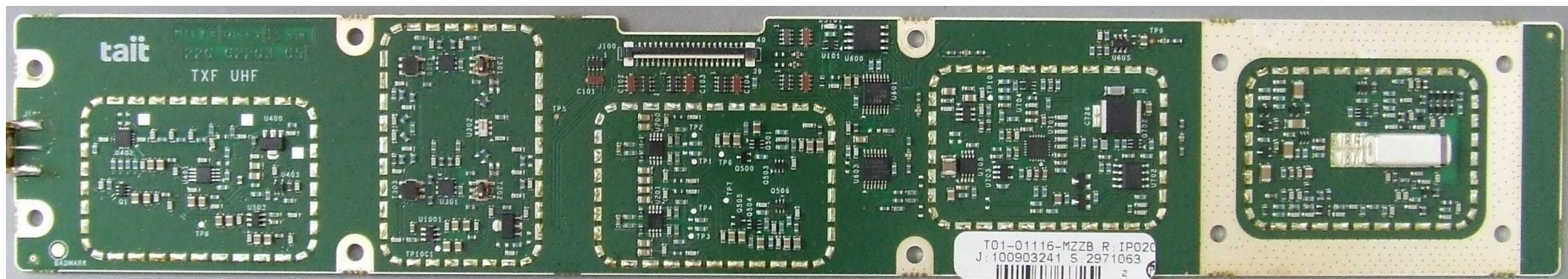
Photograph 10: Reciter TXF PCB – Top (without shields)
