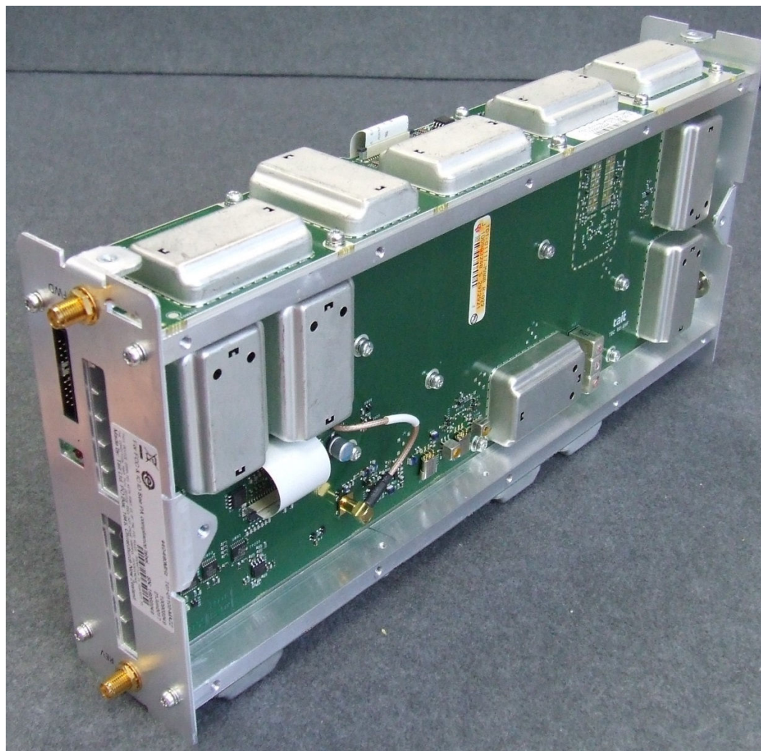
Photograph 01: Reciter module – Internal (Receiver PCB side)
