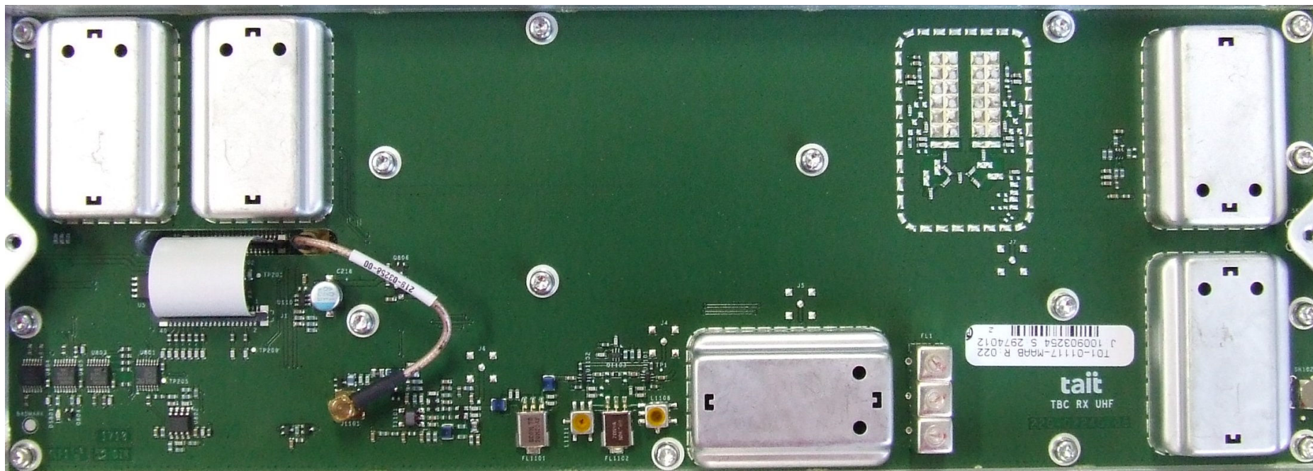
Photograph 03: Reciter Receiver PCB – Top (with shields)
