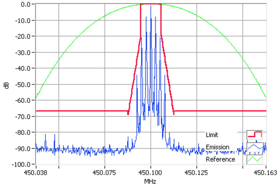
Analogue Modulation 450.1000MHz Mask D 50W RBW=100Hz, VBW=1000Hz, Detector Mode=Peak Result=Pass
