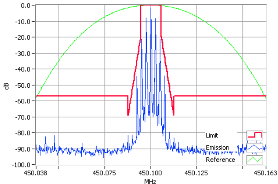
Analogue Modulation 450.1000MHz Mask D 5W RBW=100Hz, VBW=1000Hz, Detector Mode=Peak Result=Pass
