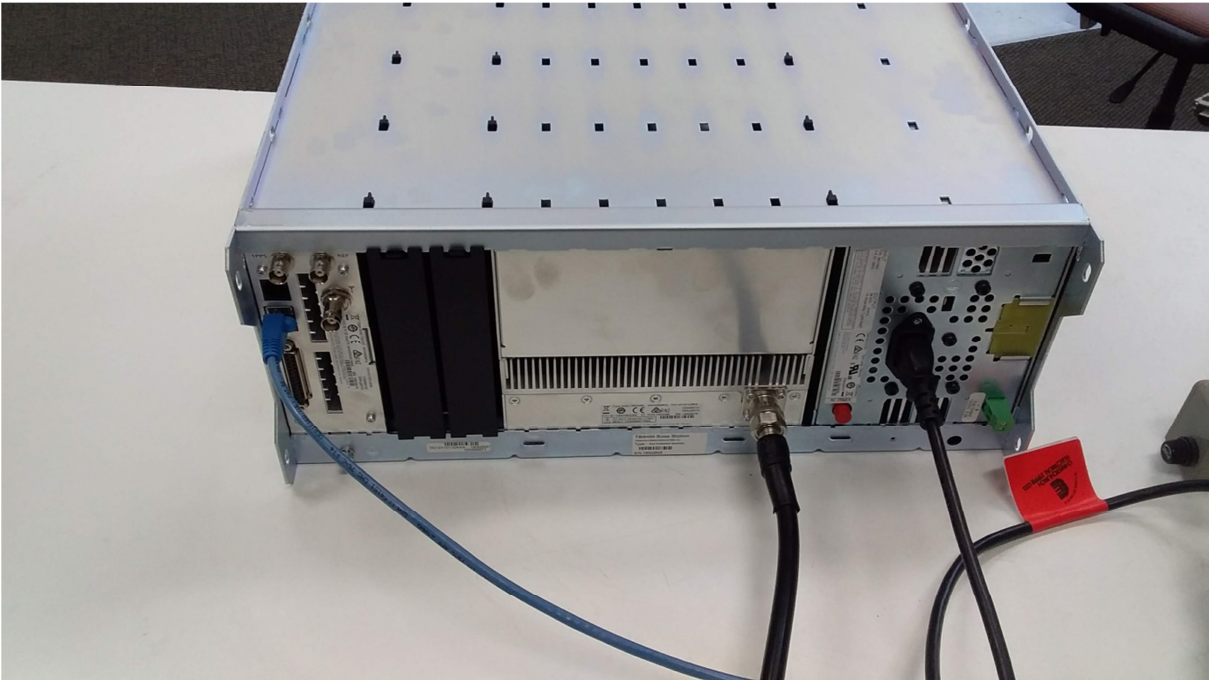
Rear Connections
