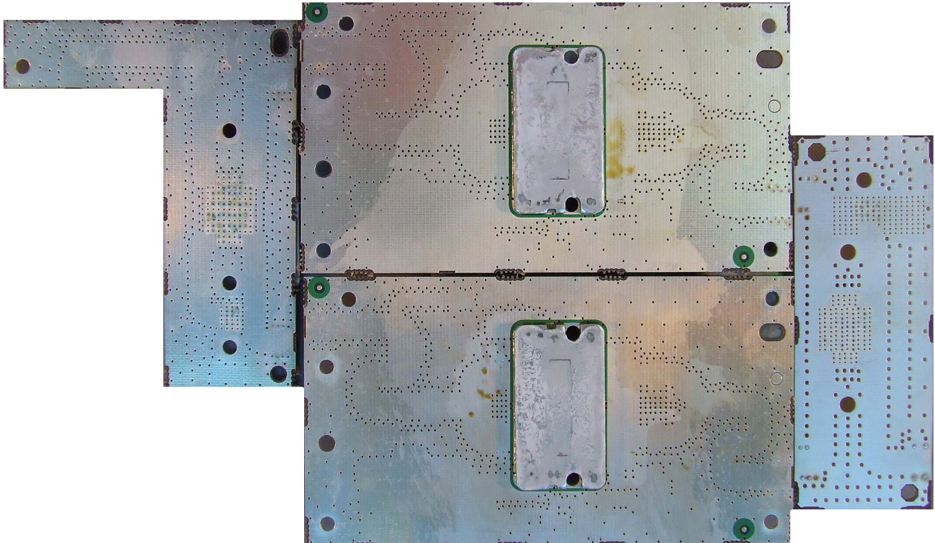
Photograph 05: 100W PA PCB - Bottom
