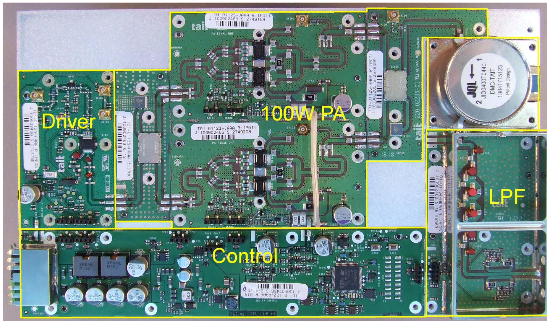
Photograph 01: 100W PA module – Internal view
