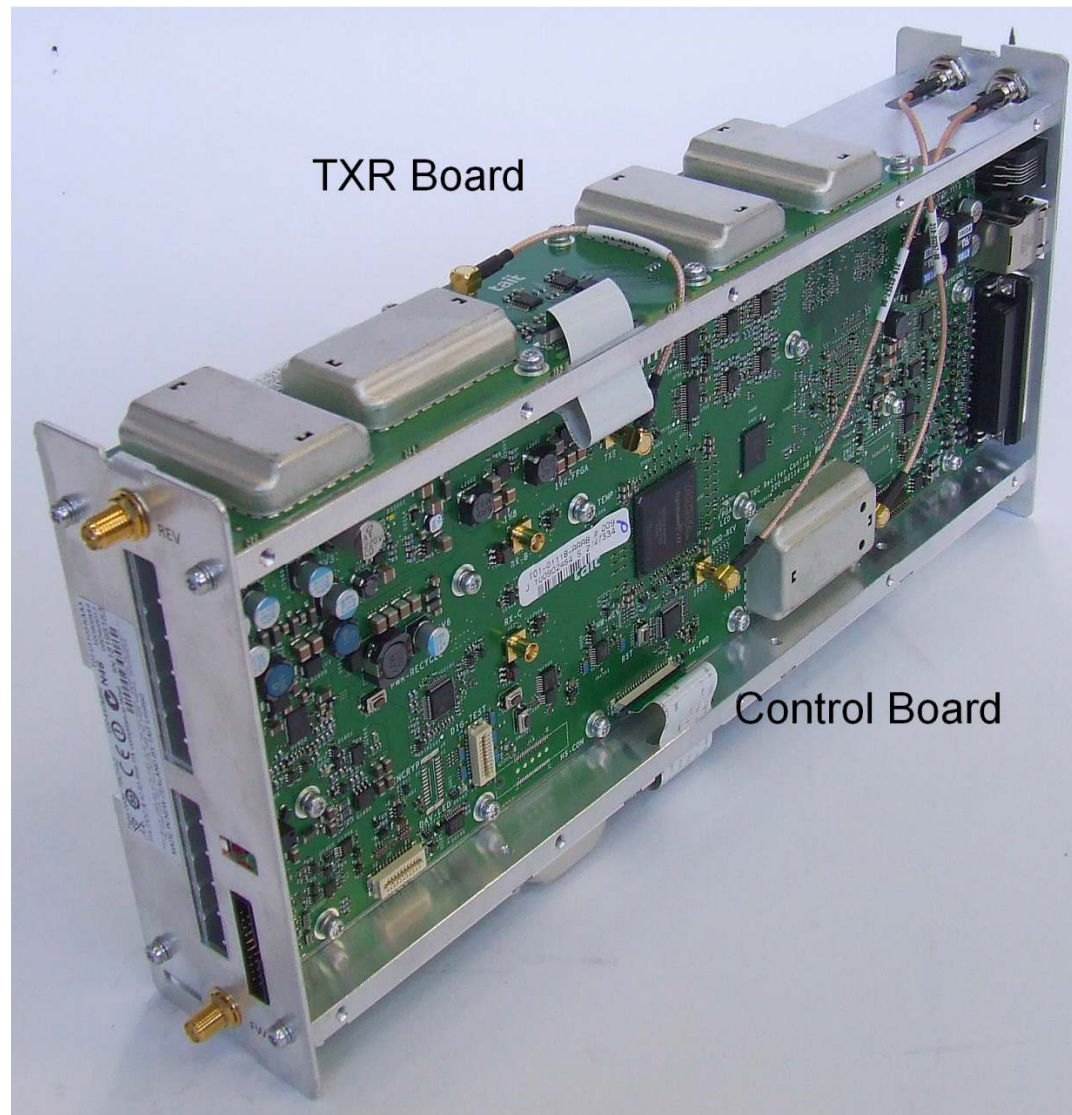
Photograph 11: Reciter module – Internal (Control PCB side)
