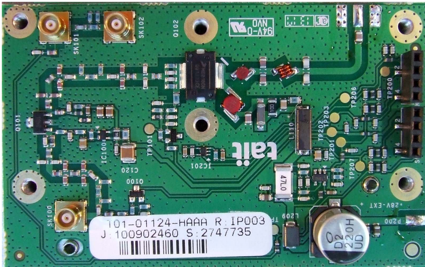
Photograph 02: PA Driver PCB - Top
