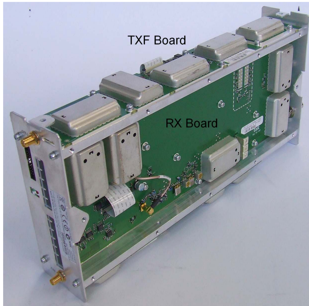
Photograph 10: Reciter module – Internal (Receiver PCB side)
