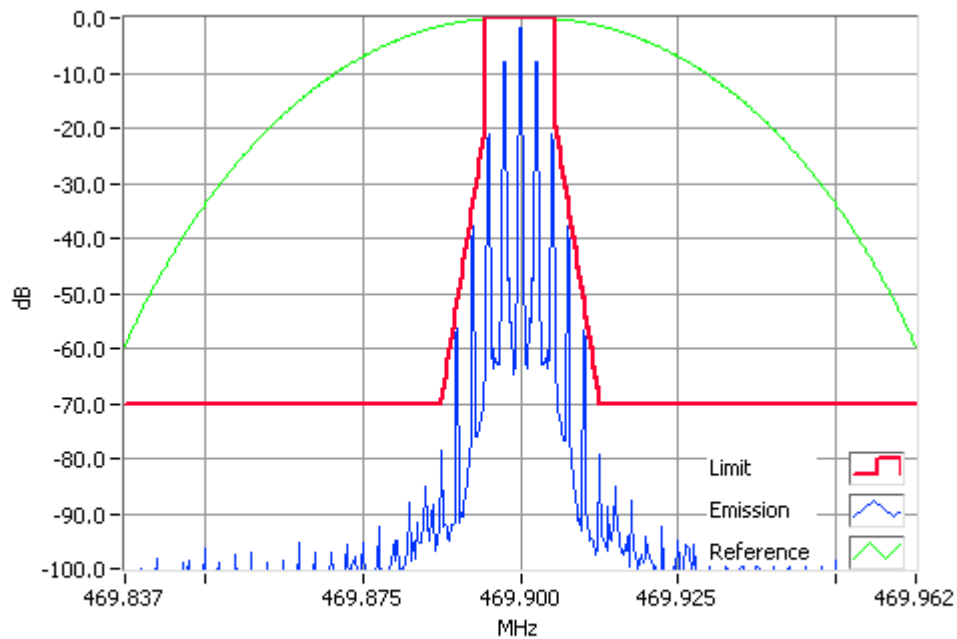
Analogue Modulation 469.9000MHz Mask D 100W RBW=100Hz, VBW=1000Hz, Detector Mode=Peak Result=Pass
