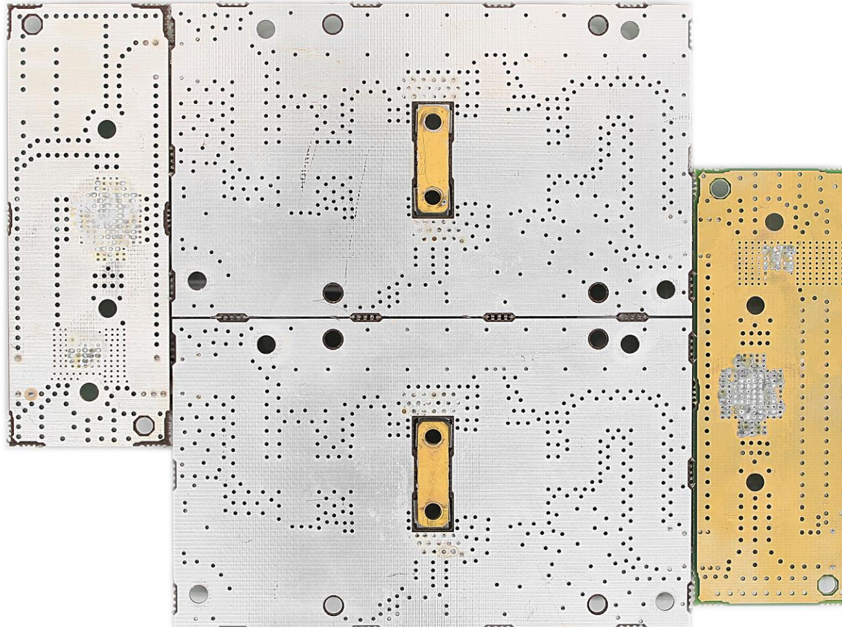
Photograph 05: 100W PA PCB - Bottom
