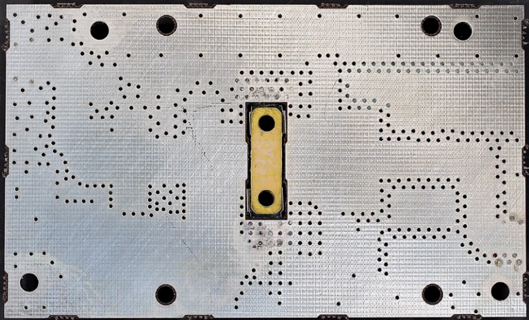
Internal100WPower Amplifier - 60W PA Board Bottom View
