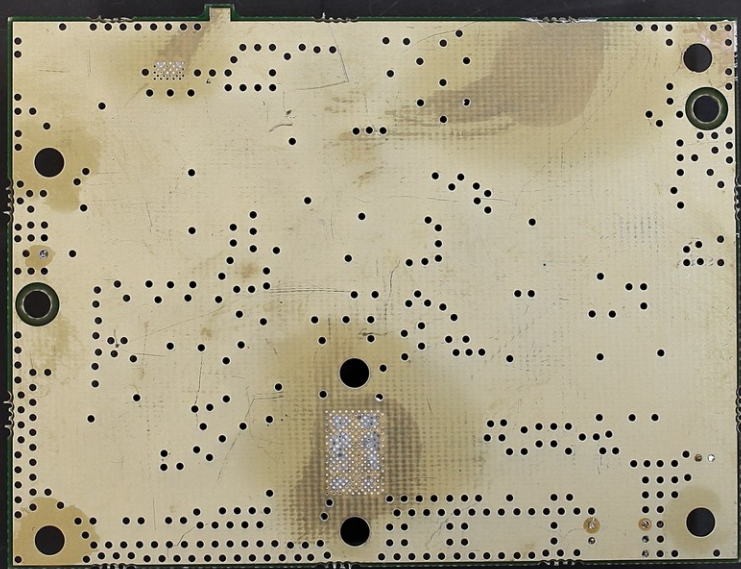
Internal 100W Power Amplifier - 6W Driver Board Bottom View
