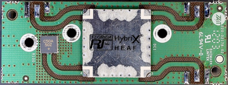
Internal 100W Power Amplifier - Combiner Board Top View
