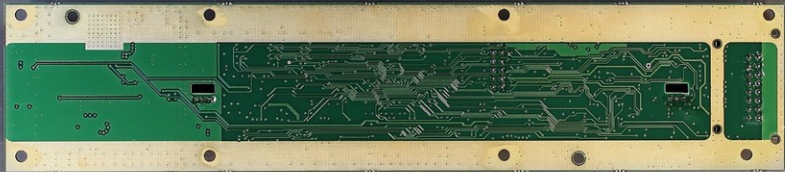
Internal 100W Power Amplifier - Control Board Bottom View
