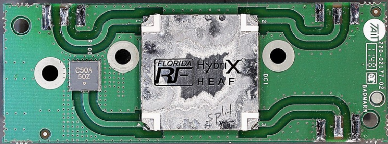
Internal 100W Power Amplifier - Splitter Board Top View
