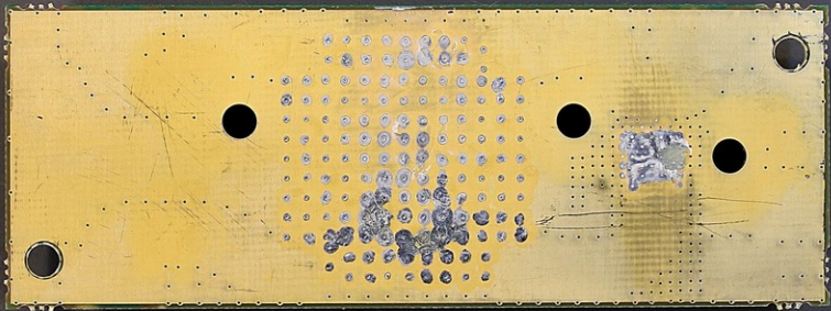
Internal 100W Power Amplifier - Splitter Board Bottom View
