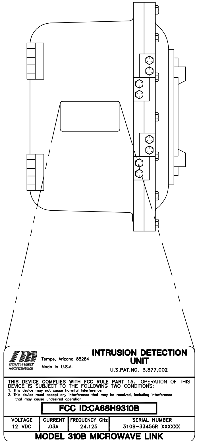
LEFT SIDE VIEW MODEL 310B-33456 TRANSMITTER & RECEIVER, EXHIBIT I
