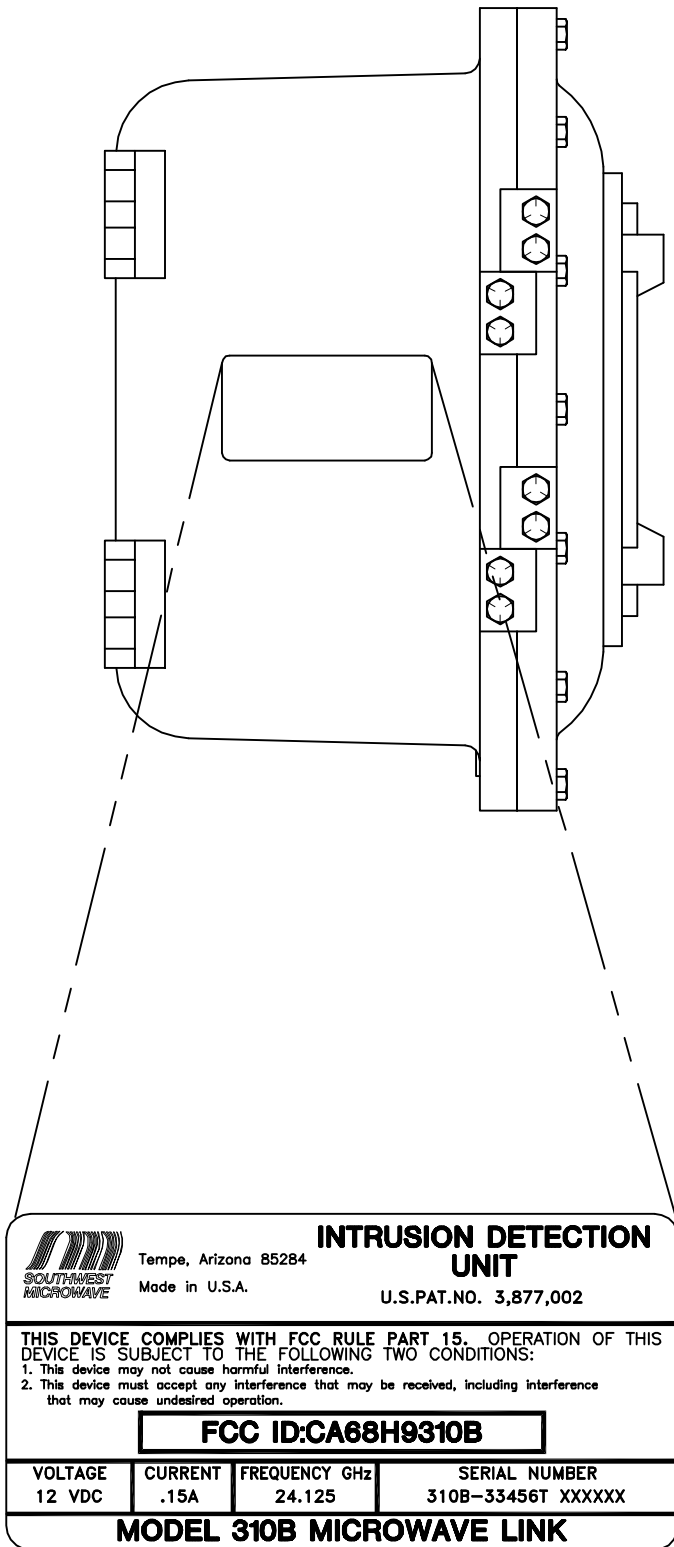
LEFT SIDE VIEW MODEL 310B-33456 TRANSMITTER & RECEIVER, EXHIBIT I
