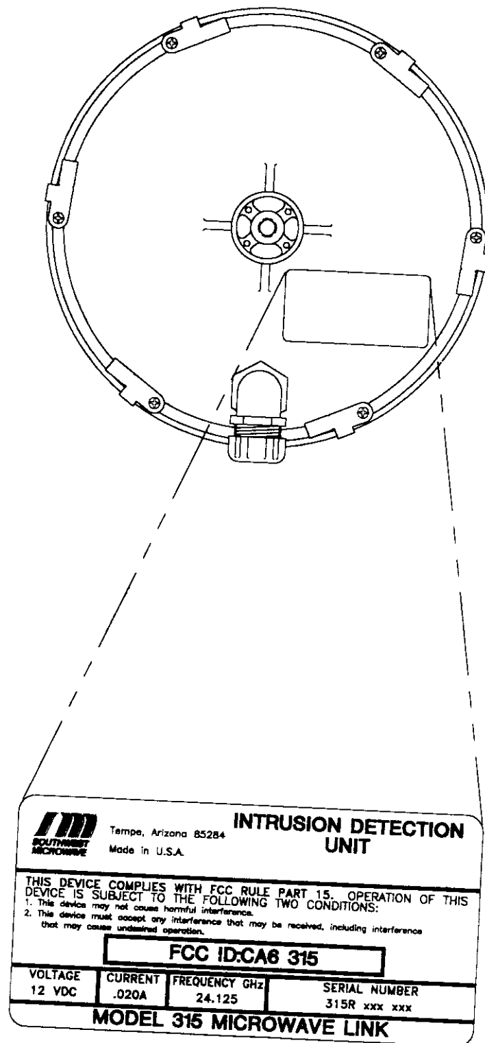
REAR VIEW MODEL 315 TRANSMITTER & RECEIVER
