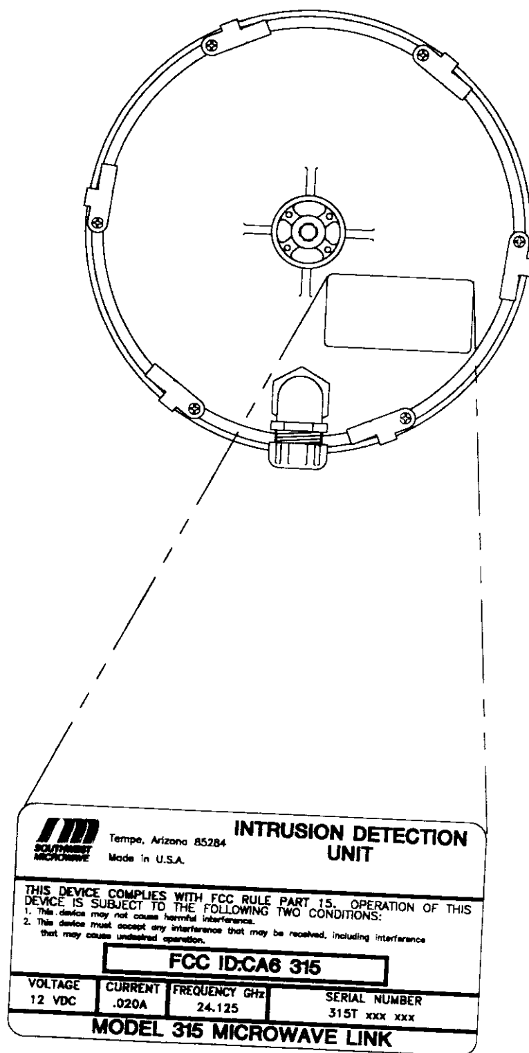
REAR VIEW MODEL 315 TRANSMITTER & RECEIVER
