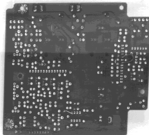
Power supply board (High voltage) CA02951-8411
