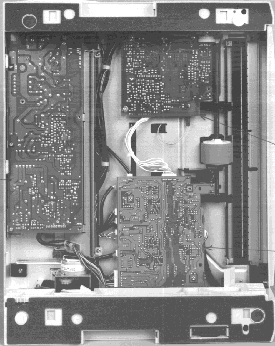
Power supply board CA02951-4274
