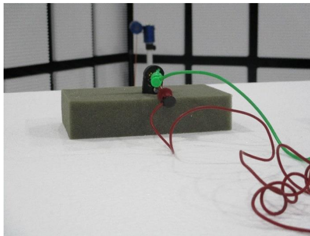
Z-ORIENTATION (Worst-case)
