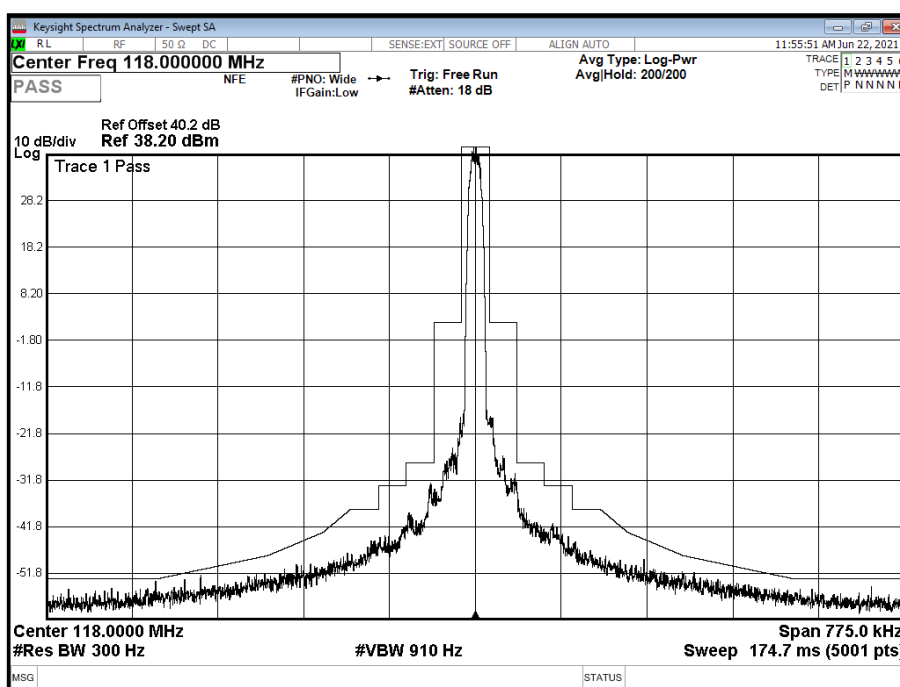
Figure 22 - 118.000 MHz, Emission Mask (within first four adjacent channels)
