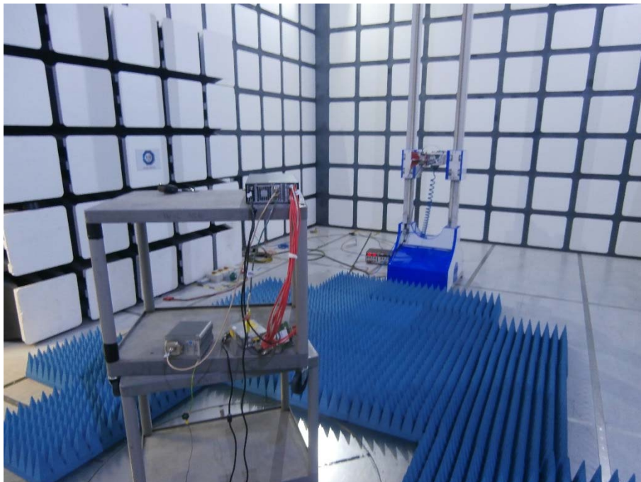
Radiated Emissions 1 GHz to 2 GHz
