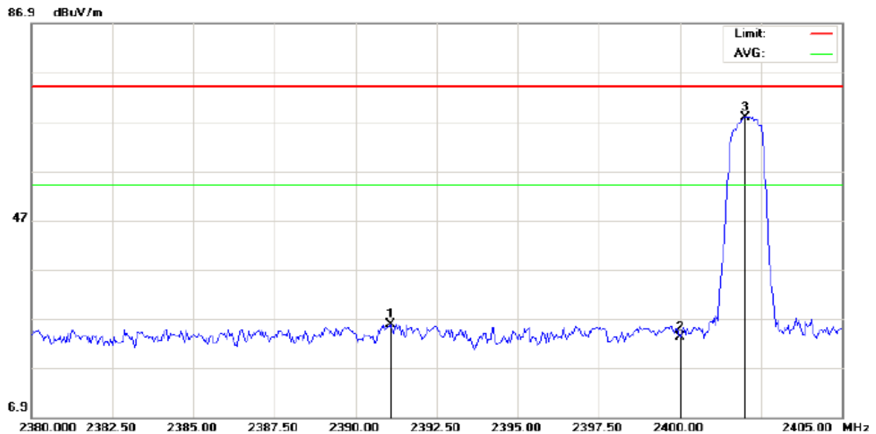
TEST PLOT OF BAND EDGE FOR LOW CHANNEL Radiated Emission Measurement
