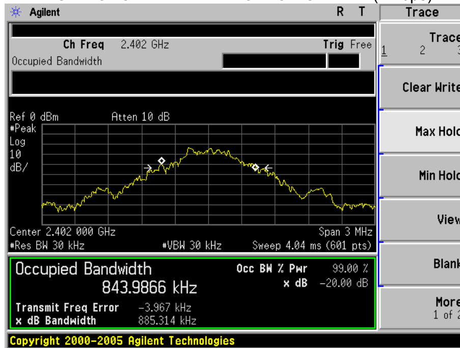
TEST PLOT OF BANDWIDTH FOR LOW CHANNEL(1Mbps)
