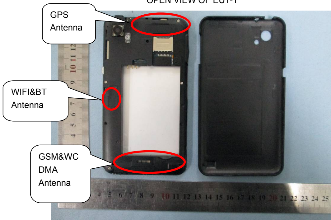
OPEN VIEW OF EUT-1
